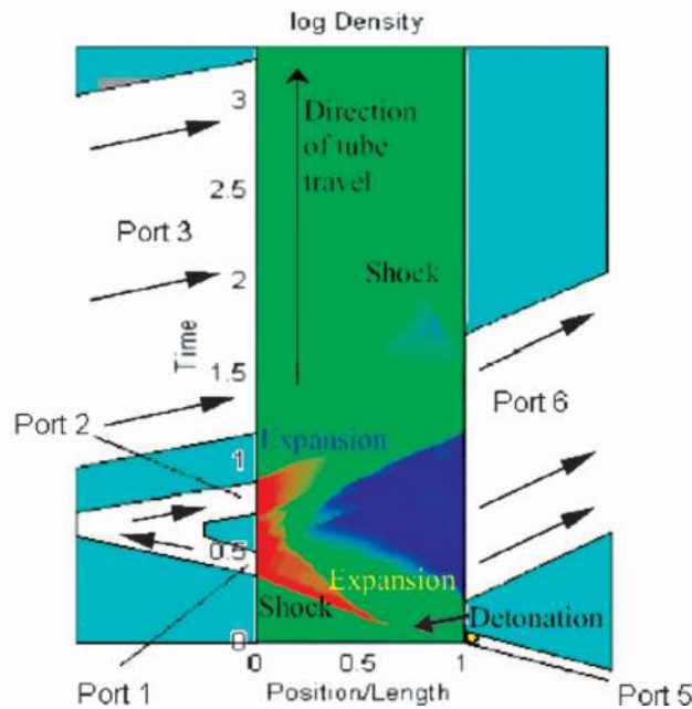
Fig. 22 Wave Rotor Pulse Detonation Engine, the “CVC” Engine, taken from Ref. [198]
