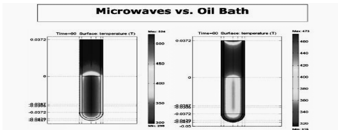
Fig:- 5. Uniform Heating through Microwave Irradiation
