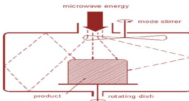
Fig:-4. Multi-mode Heating Apparatus
