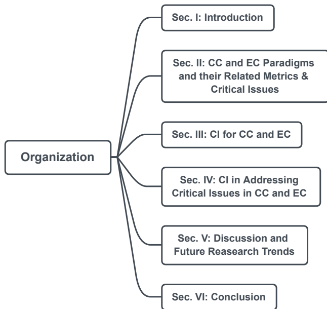
Fig. 2. Paper Organization.
