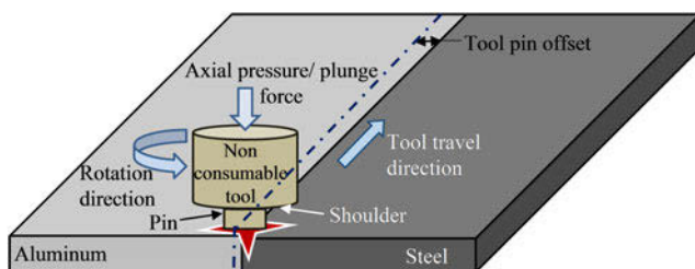
FIG. 4. Dissimilar FSW of steel to aluminum.
