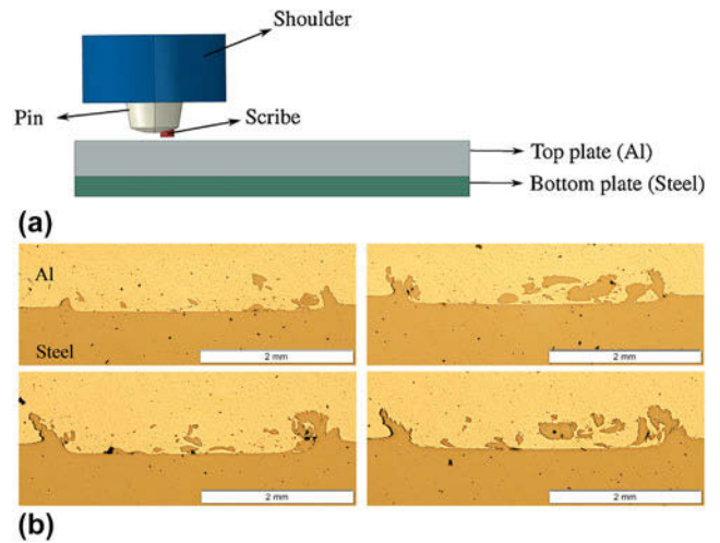
FIG. 8. (a) Friction stir scribe welding and (b) material mixing from friction stir scribe welding along the length, with permission from Ref. 144.
