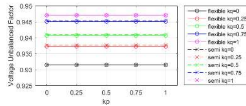
(a) Scenario I: inductive grid
