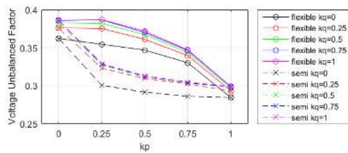
(b) Scenario II: resistive grid
