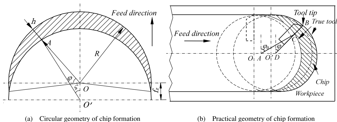
Fig. 4 Geometry of chip thickness of the milling process. f_z is the feed rate (mm/rev-tooth); \varphi is the instantaneous angle of immersion; R = D/2 , where D is the diameter of the cutter
