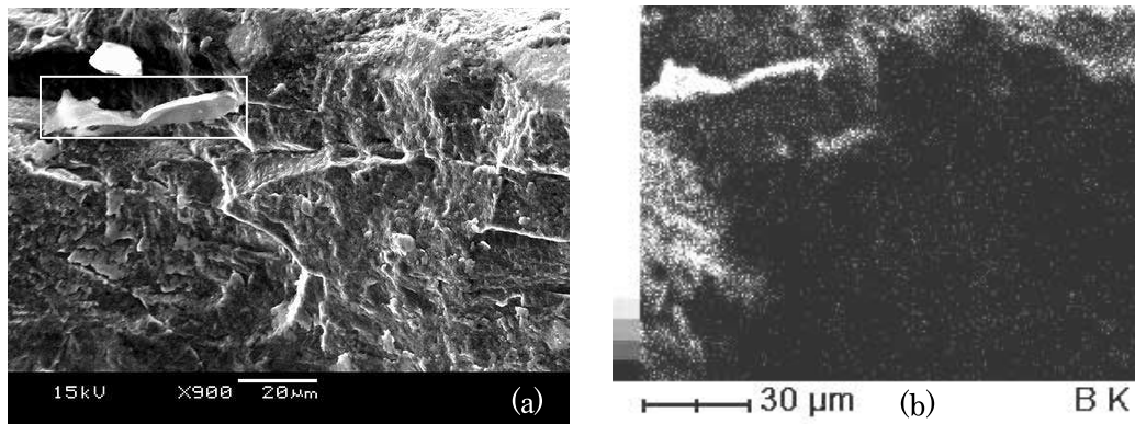
Fig. 3 SEM and EDX of the flank face (a) An enlarged rectangular region of flank face under cutting conditions of a = 0.100 mm, f = 0.10 mm/r, v = 350 m/min; (b) EDX of (a) shows the fragment in the rectangular region of Fig. 3 (a) coming from the tool material
