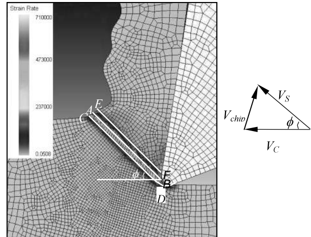
Fig. 5 Deformation zones of FEM simulation in machining of Ti6Al4V. V_C is the cutting speed, \phi is the shear angle
