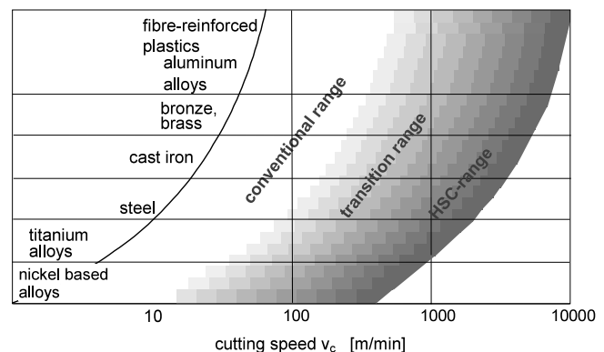
Fig. 1 Cutting speed area depends on material (1)
