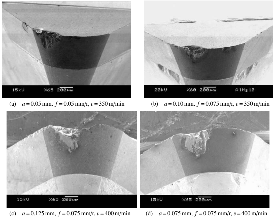
Fig. 2 SEM of the flank of BCBN tools at four different conditions where the non-uniform flank wear is the dominant wear for these four cases
