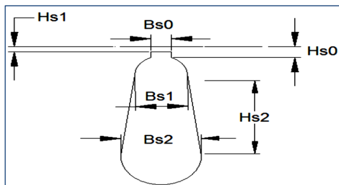
Fig. 4 Slot dimension of rotor
