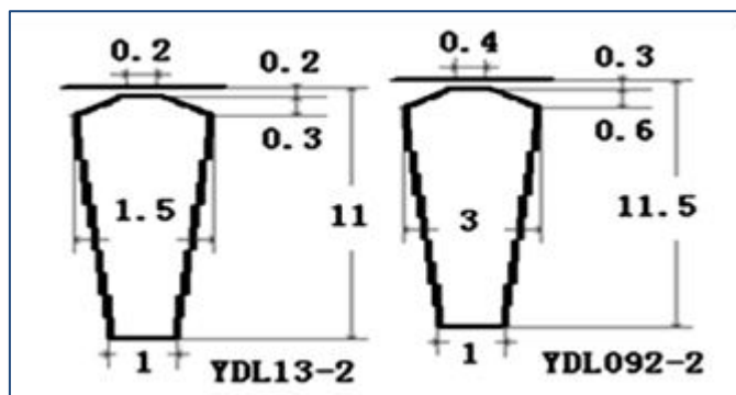
Fig. 3 Rotor slots dimensions
