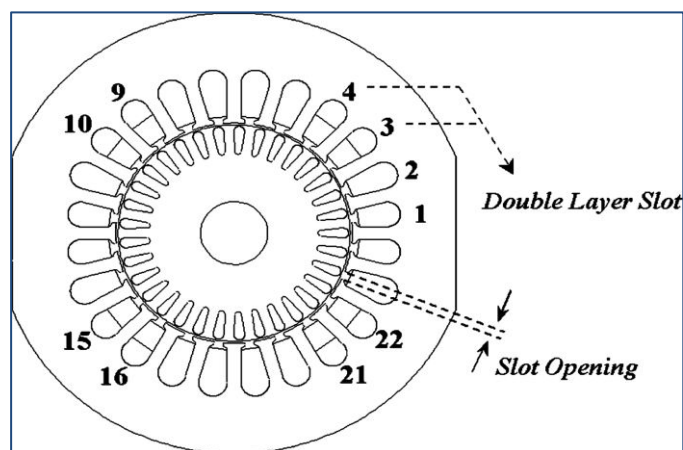
Fig. 2 Single-Phase Induction Motor with double layer stator slots
