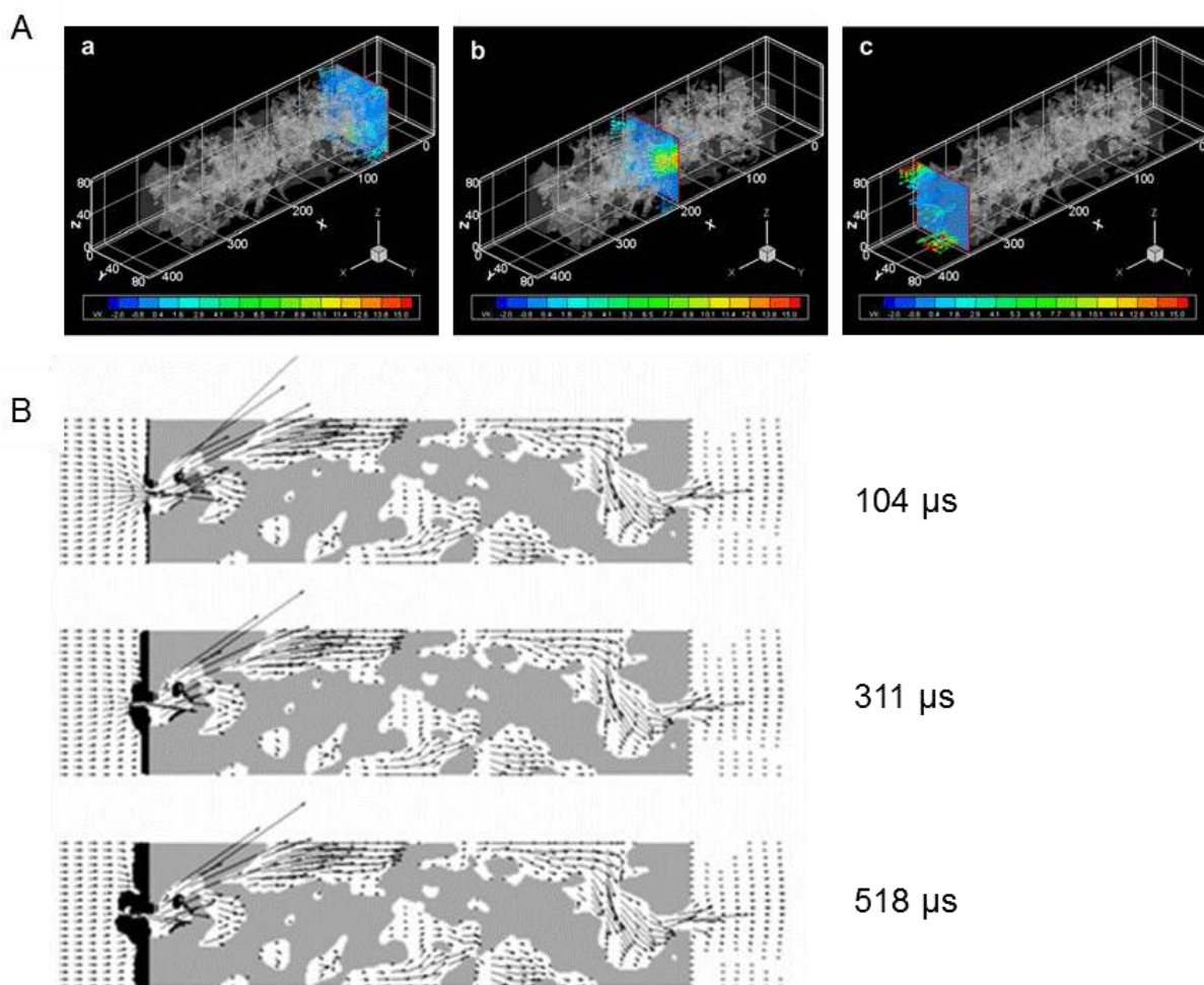
Figure 22. Flow field and filter region shown by gray region; (a) x = 40 \mu\text{m} , (b) x = 190 \mu\text{m} , and (c) x = 340 \mu\text{m} (Section A); profiles of flow field and deposited soot in x - y plane at z = 32 \mu\text{m} . Adapted from [132].
