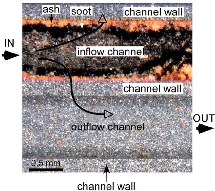
Figure 17. Representative image of two neighboring (inflow-outflow) channels (Section parallel to the flow) showing the distribution of ash (reddish) and soot (black) at the outlet-mid part of DPF. Exhaust gas flows from the left to the right and is forced through the porous walls to the adjacent outflow channels. From Ref. [123].
