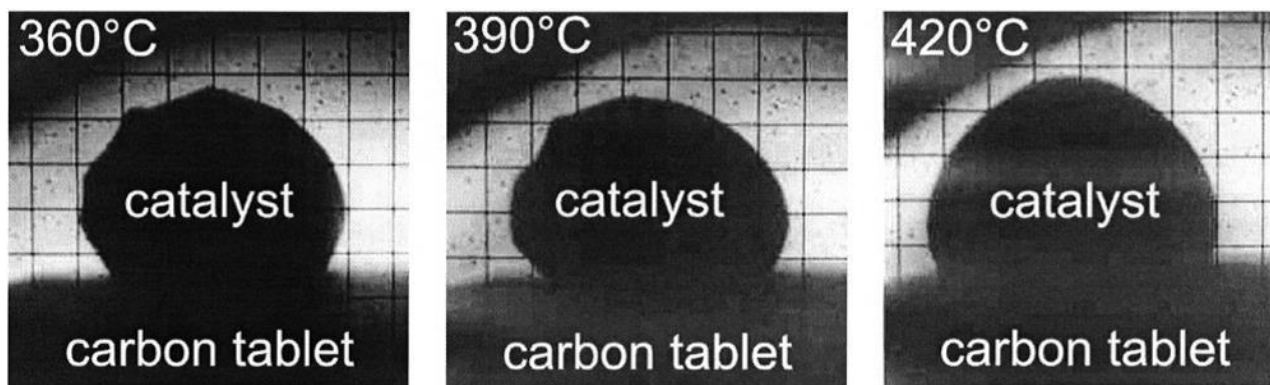
Figure 6. Images of a \text{Cs}_2\text{O}\cdot\text{V}_2\text{O}_5 sample obtained in a thermal microscope under calm air: a) 360 °C (solid catalyst); b) 390 °C (slightly before the start of eutectic liquid formation); c) 420 °C (molten catalyst). From Ref. [34].
