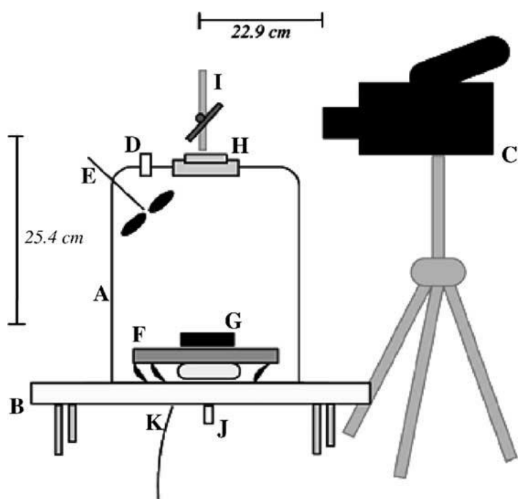
Figure 11. Scheme of the infrared (IR) catalyst characterization system: (A) outer aluminium reactor wall; (B) base plate; (C) prism DS IR camera; (D) gas inlet; (E) fan; (F) thermofoil heater; (G) combinatorial library sample holder; (H) \text{CaF}_2 window; (I) mirror and stand; (J) gas exhaust port; (K) thermocouple and furnace power leads. From Ref. [113].
