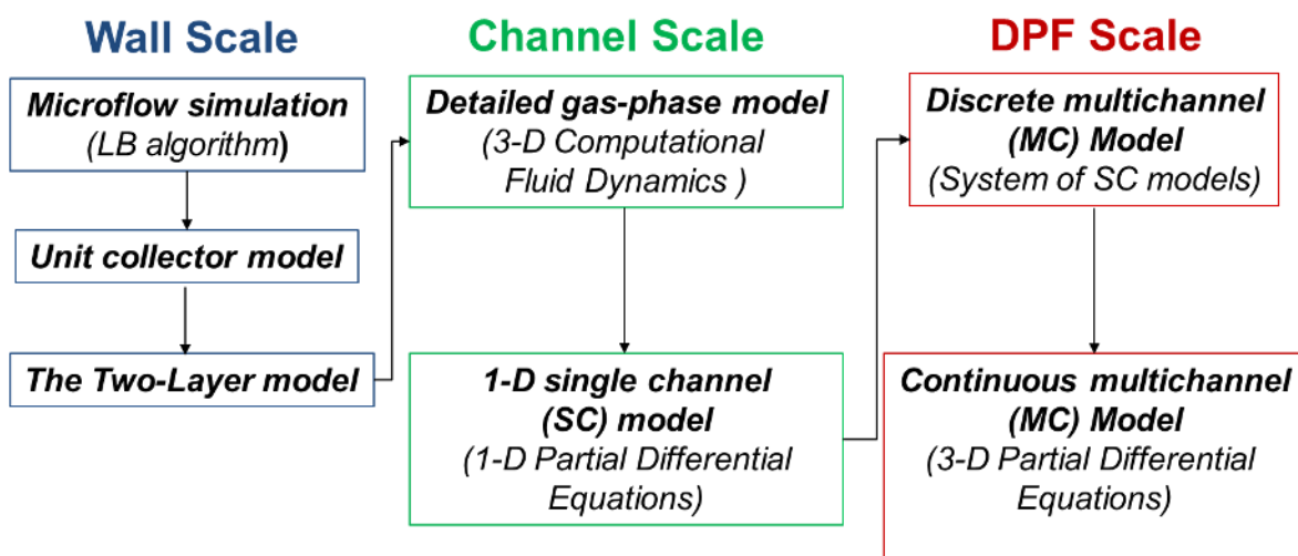
Figure 15. The hierarchical structure of sub-models at the various spatial scales employed for DPF modelling. Adapted from [17].
