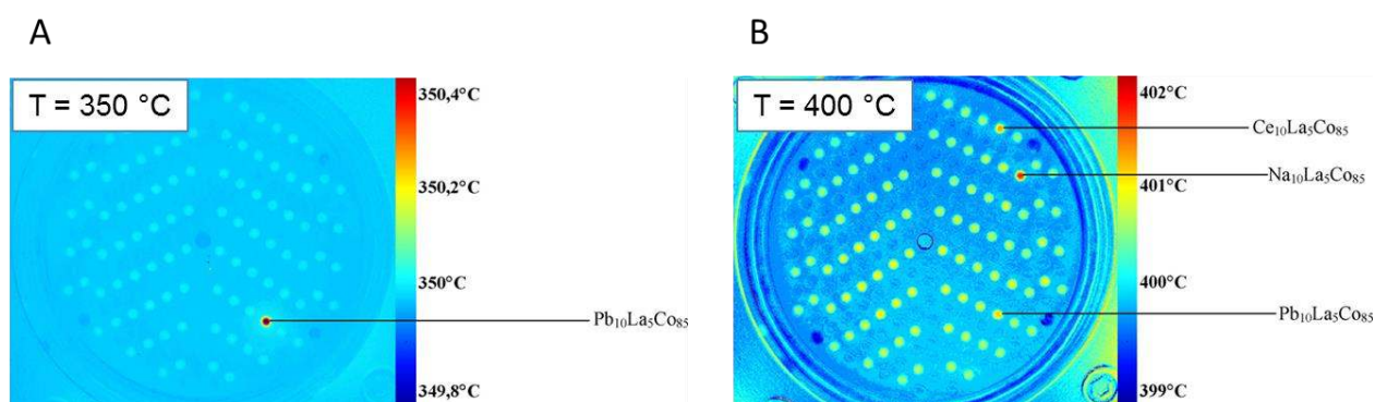
Figure 13. The emissivity-corrected IR-thermographic image of catalyst library at 350° C (Section A) and 400 °C (Section B) for soot combustion reaction. Adapted from ref [100].
