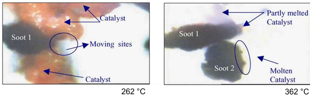
Figure 5. Microscope images of a \text{Cs}_2\text{SO}_2\text{-V}_2\text{O}_5 catalyst-soot mixture, taken at 262 °C and 362 °C. Soot 1 and 2 represent two different soot particles. The images were taken at a magnification of 50x. Adapted from [106].
