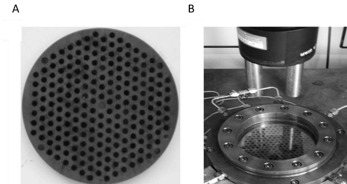
Figure 12. A slate plate for catalyst-soot samples (Section A) and IR-camera and reactor with a catalyst library for IR-thermography (Section B). From Ref. [100].
