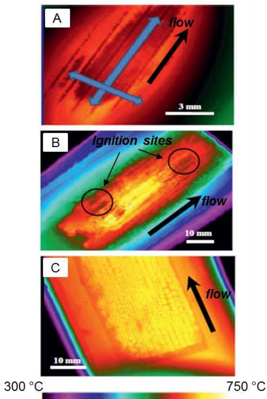
Figure 23. Thermal images of soot regeneration during combustion by: A) single ignition point; B) two-ignition points and C) uniform combustion. Adapted from [134].
