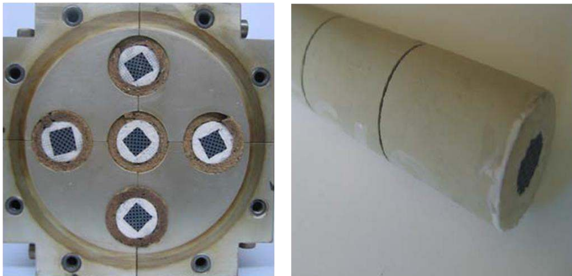
Figure 20. DPF samples mounted inside the hosting module (left) and DPF sample preparation (right) (Section A); soot layer thickness profile along the DPF channel (Section B). Adapted from [131].
