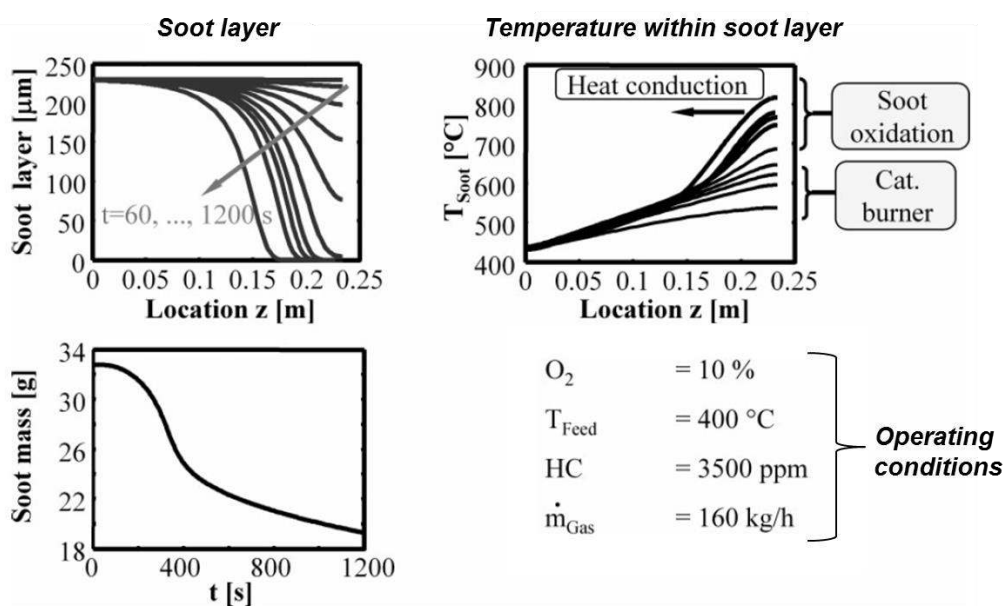
Figure 25. Regeneration of a catalytic DPF initiated by HC conversion. Initial temperature = 400 °C. From Ref. [125].
