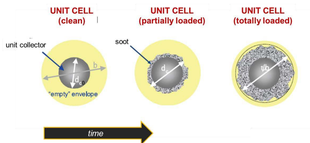
Figure 16. Unit-cell filtration model. Adapted from [116, 116b].
