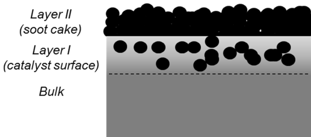
Figure 4. Scheme of the DPF wall, catalytic-coating-influenced Layer I and top Layer II which is not in the sphere of influence of the catalyst. Adapted from [102].
