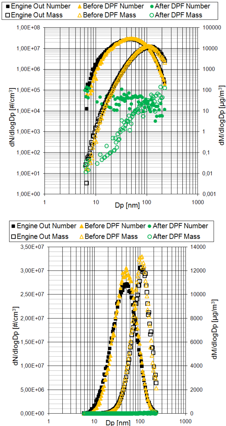
Figure 7. Particle number (left y axis) and mass (right y axis) size distributions, emitted by a light duty Diesel engine (4 stokes, 1248 cm 3 , 4 cylinders in line, maximum power of 55 kW @ 4000 rpm, bore x stroke: 69.6 mm x 82 mm, compression ratio of 16.8:1) at 1750 rpm/3.5 bar bmep. Log (top) and linear (bottom) y axis scales. Adapted from [110].
