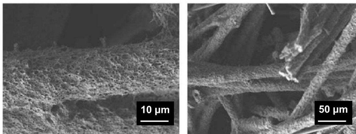
Figure 3. SEM images of a nanofibrous \text{LaMnO}_3 catalyst on silica fibers. Adapted from [94].
