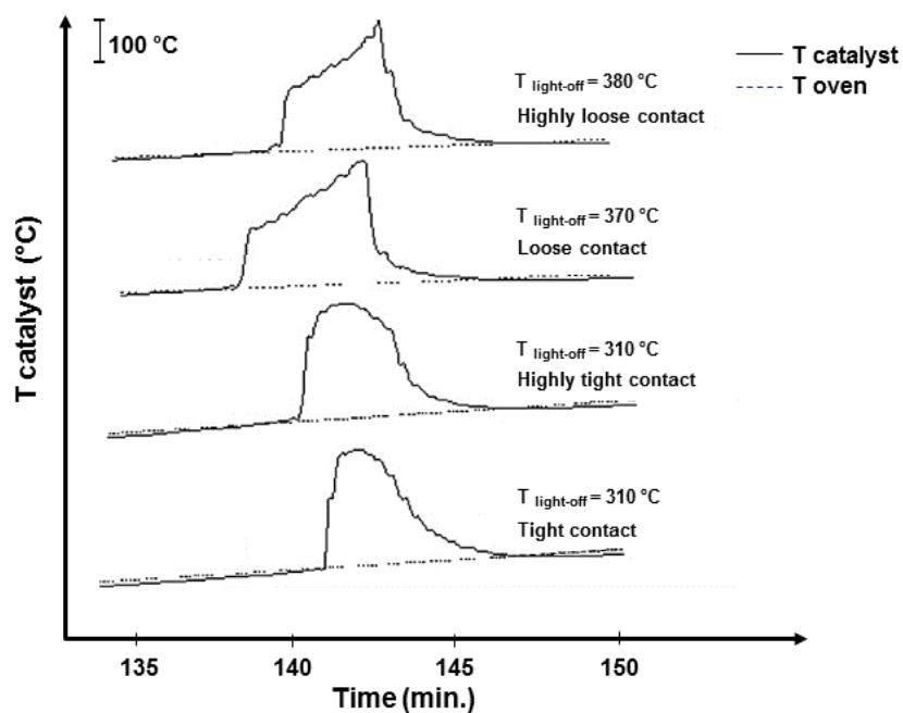
Figure 8. Light-off for soot combustion as a function of the contact type between the catalyst and the soot: 40 mg soot/400 mg CeO 2 under 40 mL/min 50% O 2 /Ar. Adapted from [111].
