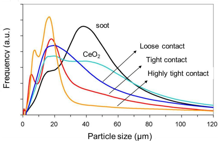
Figure 9. Particle size distribution of soot, Ceria and soot-Ceria mixtures in “loose”, “tight” and “highly tight” contact conditions. Adapted from [111].
