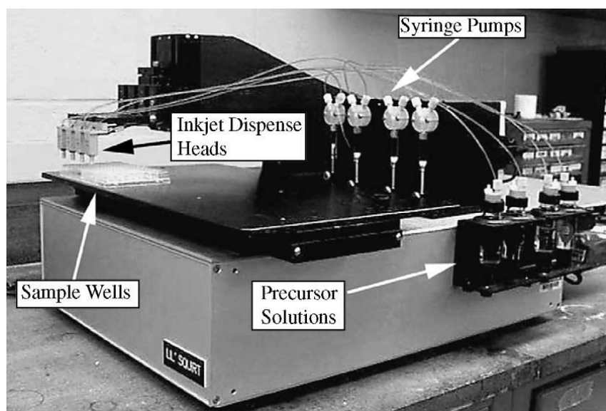
Figure 10. Inkjet dispensing system used for library synthesis. From Ref. [113].
