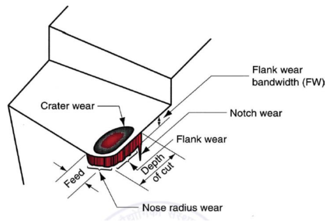
Figure 1. Types of tool wear [23]
