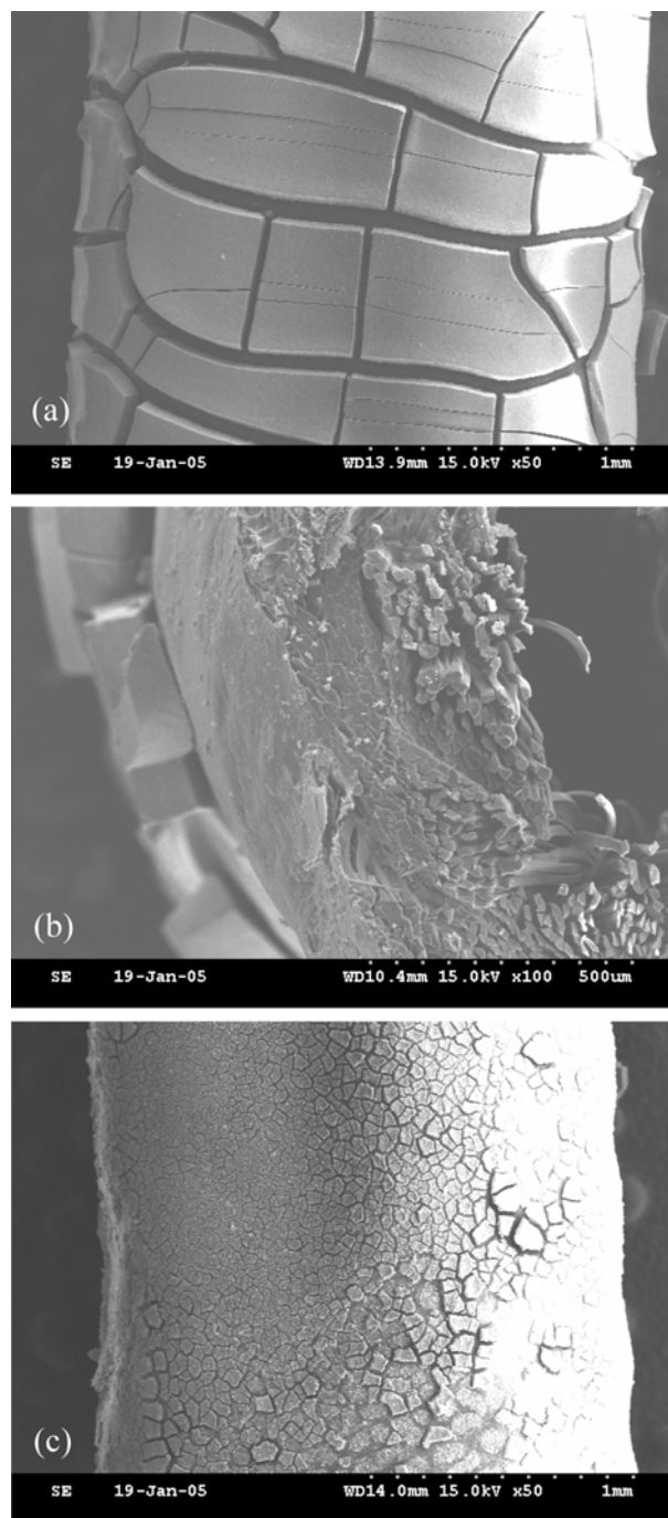
Fig. 10. SEM images of the membrane used in the separation of TiO 2 particles in suspension by photocatalytic membrane hybrid system (a) cake deposit on the membrane surface after photocatalytic process, (b) cross section of the membrane showing the thickness of the cake deposit (c) particle deposits on membrane surface after two stage coagulation and sedimentation.
