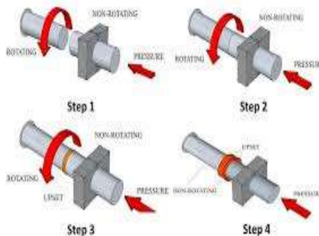
Friction Welding
