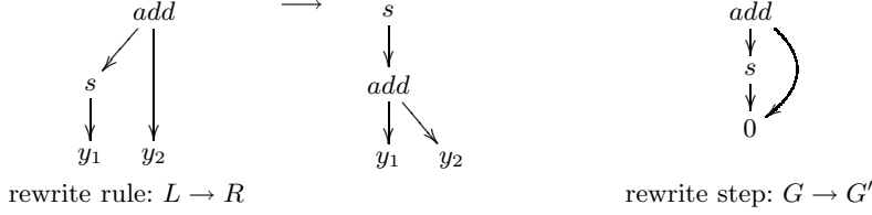
Figure 14. Example of rewriting in a TGR.
