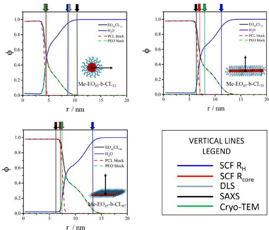
Figure 4. SCF concentration profiles for the self-assembled structures of some of the synthesized copolymers. The plots show how the volume fraction ( \phi ) of a certain component change as function of the distance from the center ( r ) of the structure. Predicted and experimentally measured sizes are depicted as vertical lines of different colors
