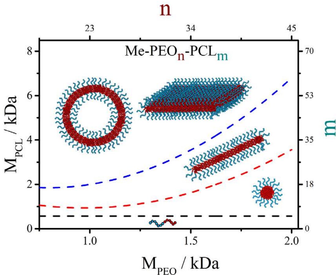
Figure 2. Morphology phase diagram for PEO-PCL block copolymers in water at T=20\text{ }^{\circ}\text{C} obtained by SCF. The dashed curves separate the stability regions for different morphologies. The composition of the copolymers are expressed in terms of mass ( M ) and block lengths ( n and m ). The region below the black dashed line indicates when the copolymer is soluble. The region between the black and the red dashed curve indicate the stability region for spherical micelles. The region between the red and the blue dashed curve cylindrical micelles are stable. The region above the blue dashed curve corresponds to the formation of vesicles or flat bilayers.
