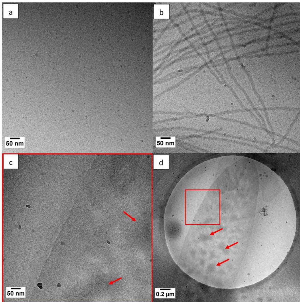
Figure 5. Cryo-TEM images of (a) EO 45 -b-CL 12 ; images show spherical micelles with a radius of 4.5±1 nm. (b) Me-EO 45 -b-CL 35 ; images display cylindrical micelles with a cross sectional radius of 8±1 nm surrounded by minor ice contamination. (c,d) Me-EO 45 -b-CL 87 ; on image c multiple leaf shaped bilayer, the dominant observed morphology, can be seen. At high magnification (c) an edge with thickness 14±9 nm can be observed. Further, in image (d) centre-left a seemingly micellar packed spherical structure can be observed. Red arrows indicate some of the areas with darker contrast, attributed to the presence of crystalline domains.
