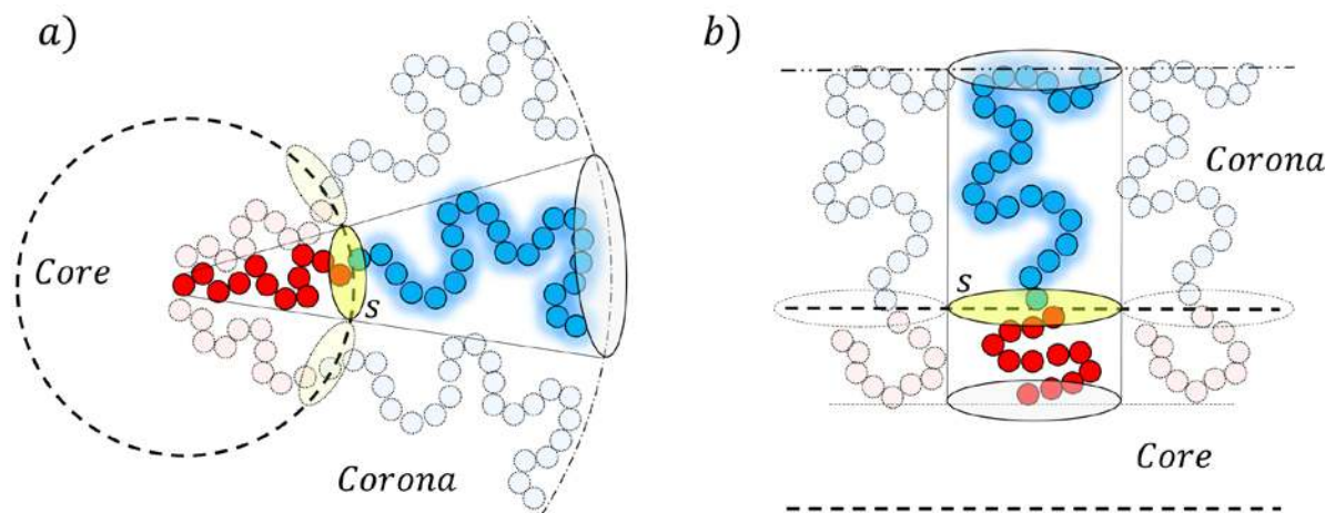
Figure 1. Schematic representation of a block copolymer in a spherical micelle (a) and a flat bilayer (b). The Interfacial area of the chains is noted in yellow.
