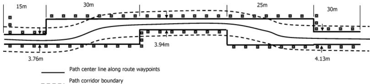
Figure 30. Blind and perception assisted path tracking route through modified ISO-3888-1 test track.
