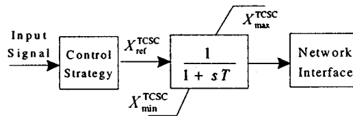
Fig. 3. TCSC model as damping controller.
