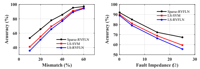
Fig. 3. Comparison of SC fault detection accuracy by Sparse-RVFLN, LS-SVM, and LS-RVFLN.
