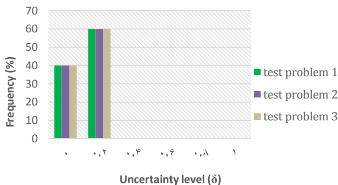
Fig. 11. The uncertainty levels' frequencies under different realizations
