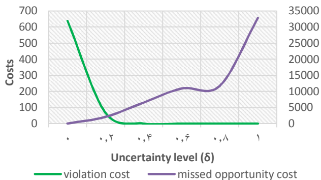
Fig. 8. Violation cost versus missed opportunity cost for the first test problem
