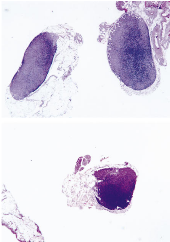
Figure 2. Lt\beta^{-/-}tnfr1^{+/+} mice have defective MLN development. Lt\beta^{-/-}tnfr1^{-/-} mice completely lack MLNs and Lt\beta^{-/-}tnfr1^{+/+} littermates have MLN of apparently normal size and number (top), but Lt\beta^{-/-}tnfr1^{+/+} littermates most often have only a single, small MLN (bottom). Hematoxylin and eosin histology; original magnification: \times 15 .
