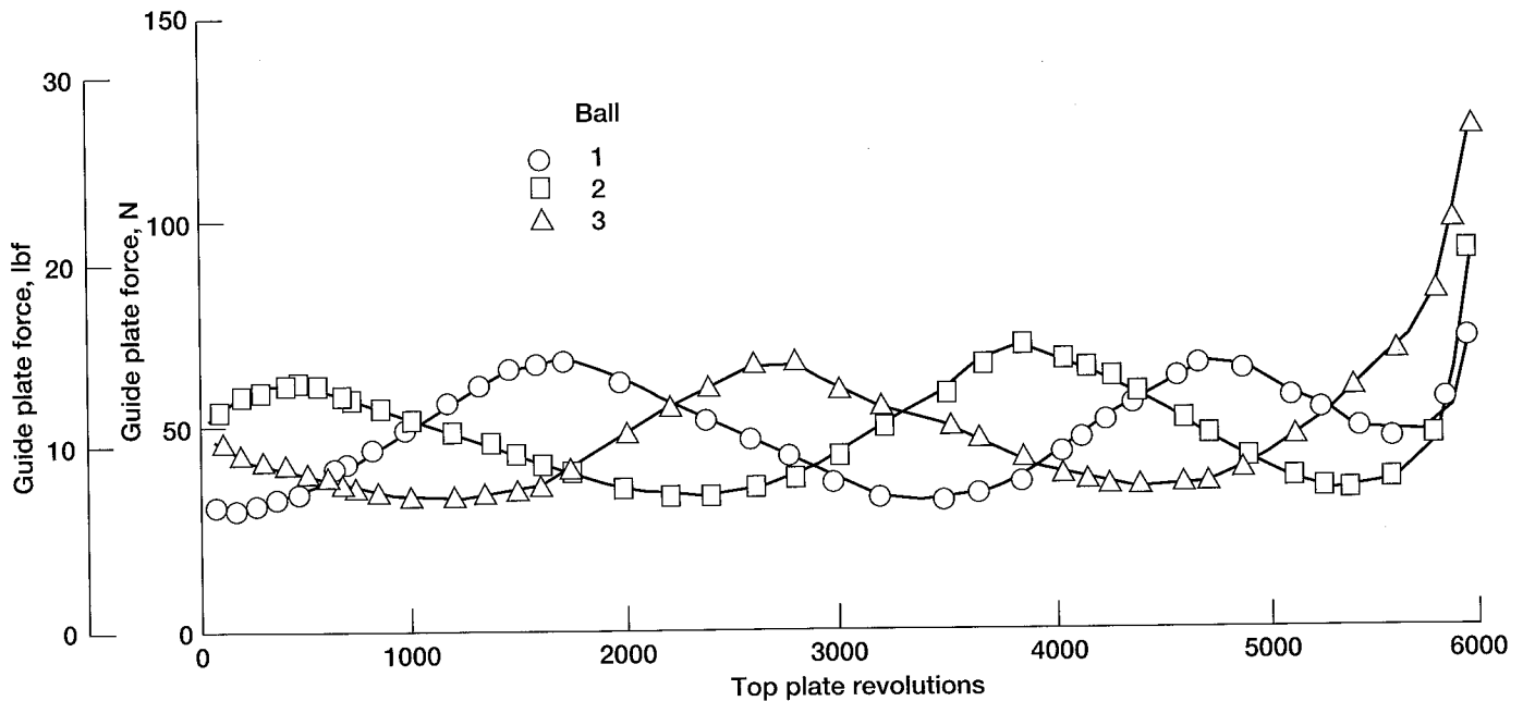
Figure 9.—Contact force on guide plate for complete test with Fomblin Z-25. The force due to each ball is oscillatory as a function of top plate revolutions. Note abrupt increase at \approx 5500 revolutions.
