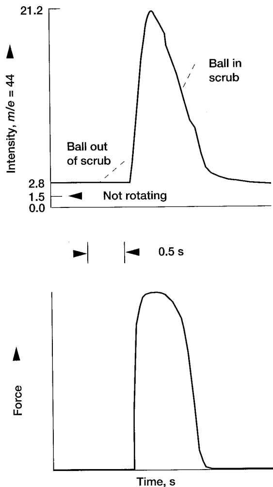
Figure 6.—Upper trace shows experimental intensity of residual gas analyzer signal for m/e = 44 ( \text{CO}_2 ); lower trace shows contact force on guide plate as ball lubricated with Fomblin Z-25 passes through scrub region.
