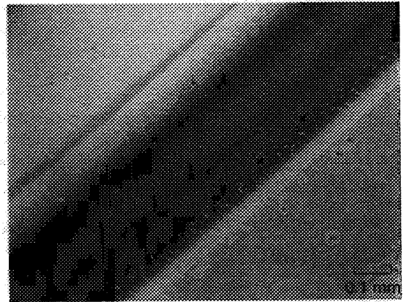
Figure 12.—Optical micrograph of track on bottom plate after completion of test with Fomblin Z-25.
