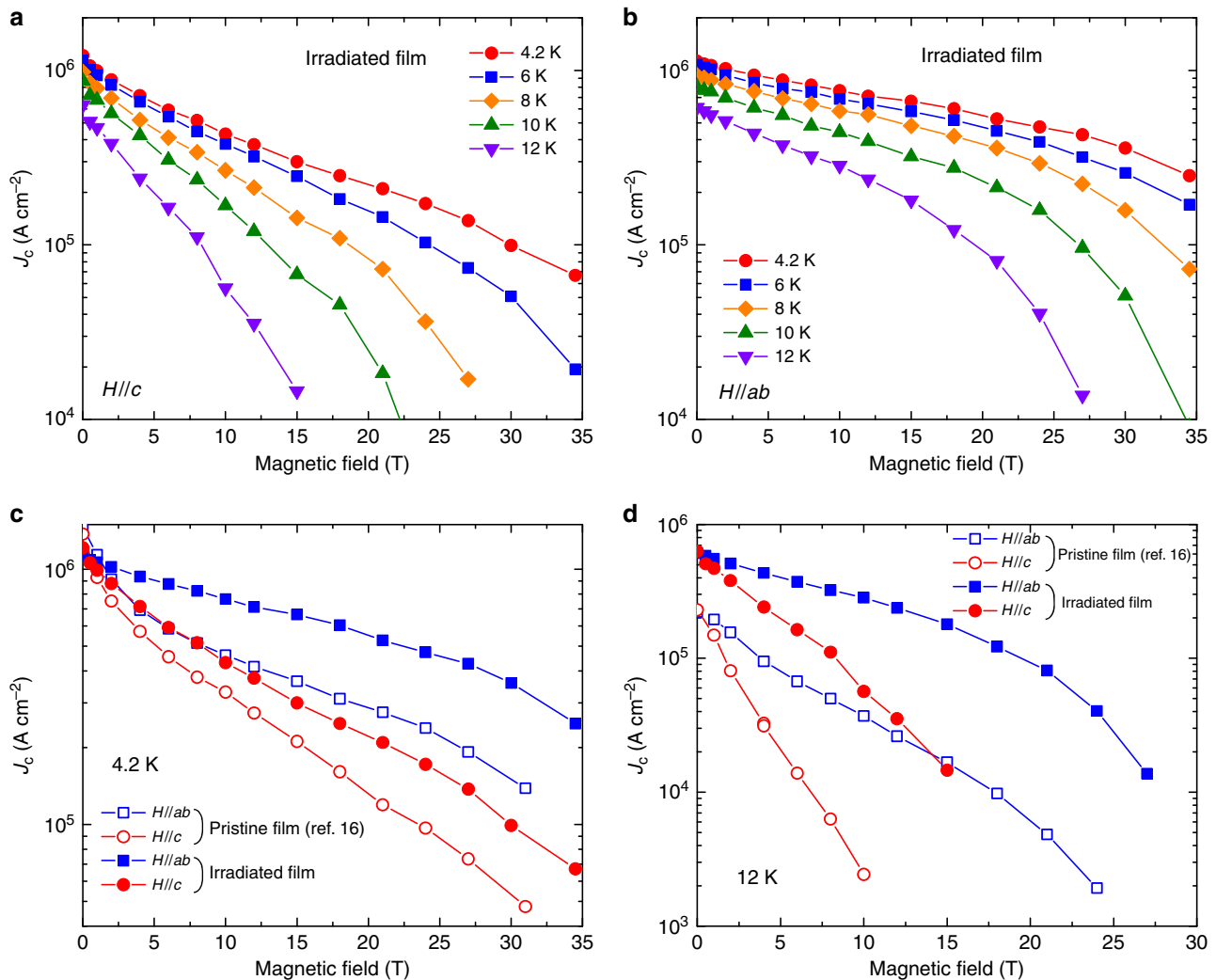
Figure 6 | High-field critical current density up to 34.5 T. (a,b) J_c(H) for proton-irradiated FST film with 1 \times 10^{15} p cm -2 dose at different temperature up to 34.5 T with H//c and H//ab, respectively. (c,d) J_c(H) for the irradiated FST film up to 34.5 T compared with the pristine FST film 16 at 4.2 and 12 K, respectively.
