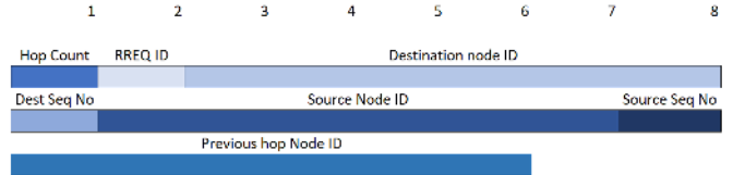
Fig. 1. RREQ packet format
