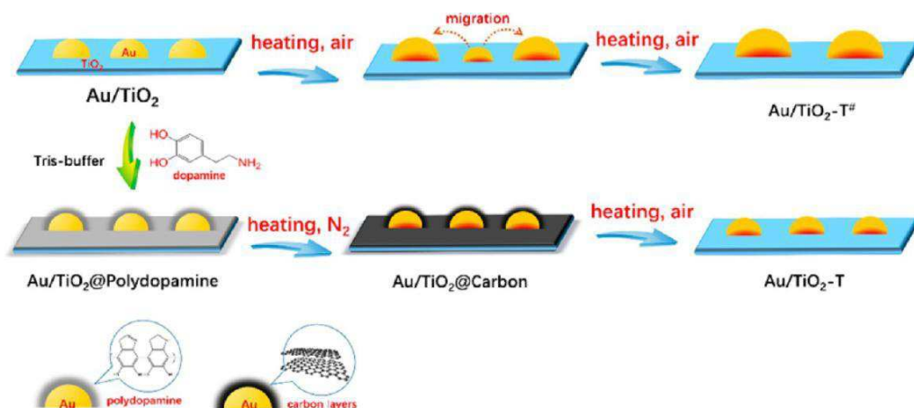
Scheme 1. Illustration Depicting the Construction of a Dopamine-Derived Layer Architecture for the Annealing Engineering of Au Nanocatalysts with High Thermal Stability
