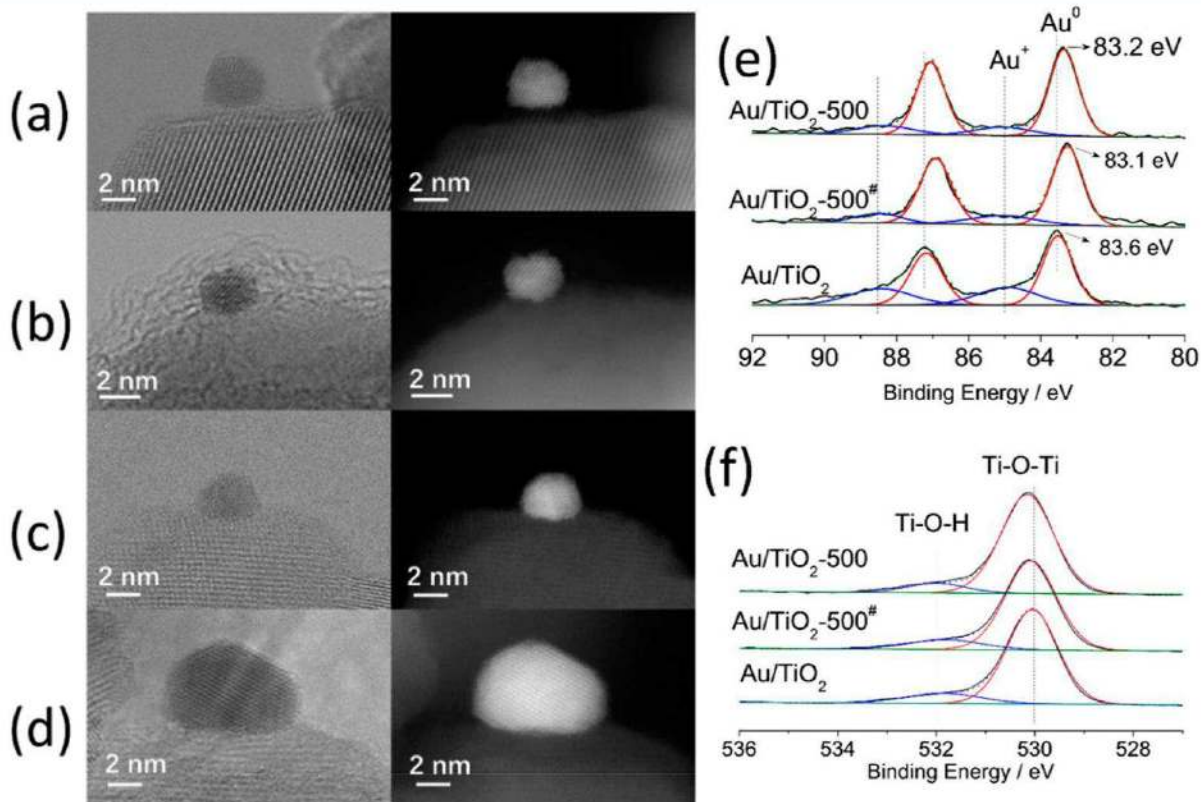
Figure 5. BF-STEM and HAADF-STEM images of (a) Au/TiO 2 , (b) Au/TiO 2 @Carbon, (c) Au/TiO 2 -500, and (d) Au/TiO 2 -500 # , respectively. (e) Au 4f and (f) O 1s XPS spectra of Au/TiO 2 , Au/TiO 2 -500, and Au/TiO 2 -500 # .
