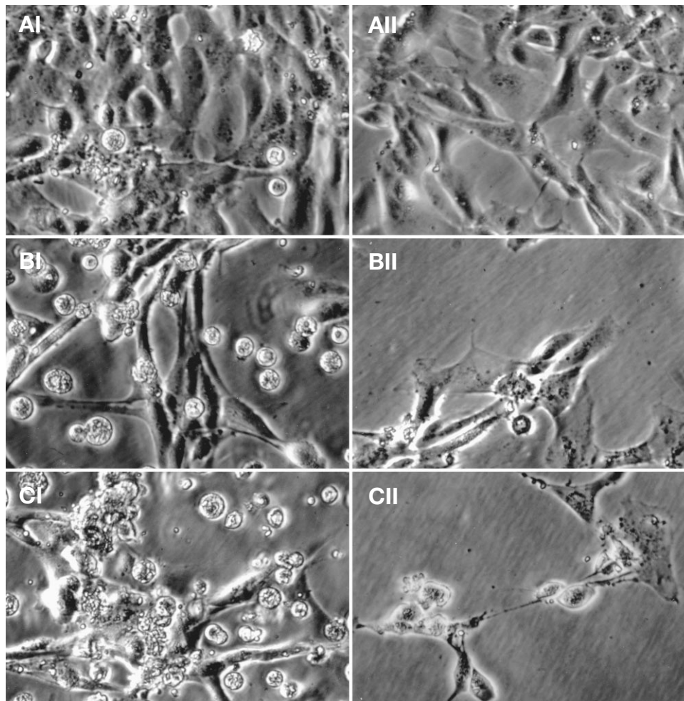
Fig. 2. TO cells after infection with virus supernatant containing ISAV. Virus supernatant had been frozen, centrifuged, filtered and diluted 1:100. (AI) 3 d after infection. Note presence of a few round cells in the medium and areas without cells. (AII) Same preparation as in (AI) but growth medium has been removed. Note presence of numerous vacuoles in neighbouring cells, the first visible sign of CPE. (BI) 6 d after infection. Note many rounded cells in the medium. (BII) Same preparation as in (BI) but growth medium has been removed. Note extended cell-free areas. (CI) 9 d after infection. Note large number of cells and amount of cell debris in the growth medium. (CII) Same preparation as in (CI), but growth medium has been removed. Magnification, \times 200
