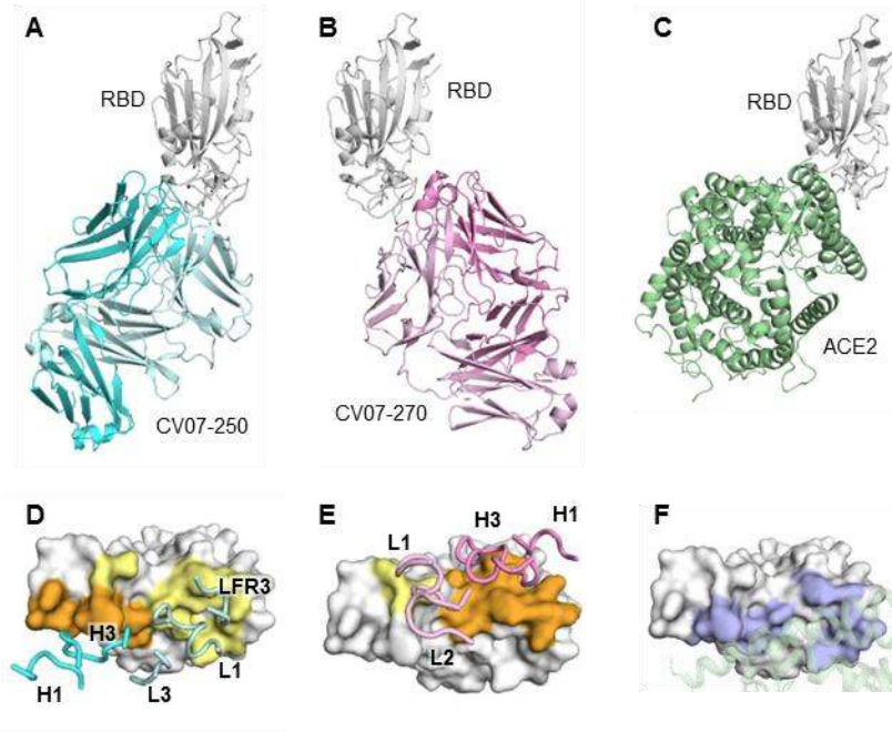
Fig. 3 | Crystal structures of mAbs in complex with SARS-CoV-2 RBD.
