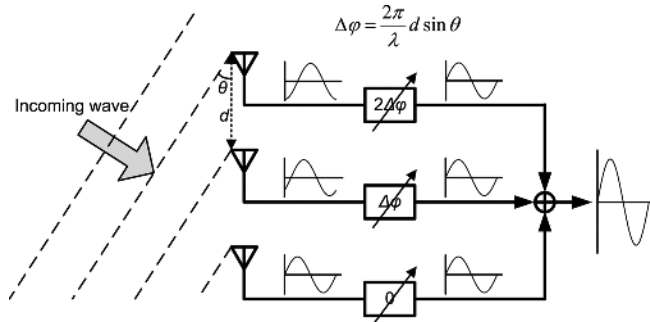
Fig. 1. Basic phased-array receiver configuration.
