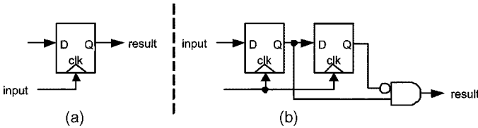
Fig. 10. Traditional methods to detect signal rising edge.
