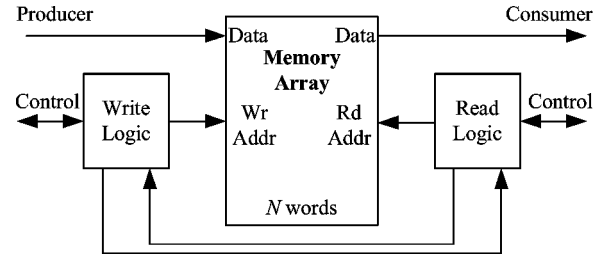
Fig. 3. Circular FIFO block diagram.
