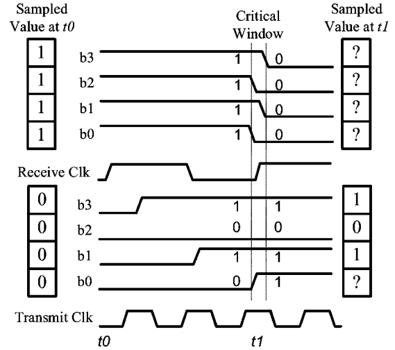
Fig. 5. (top) Sampling of a multibit transition word and (bottom) a single-bit transition word.
