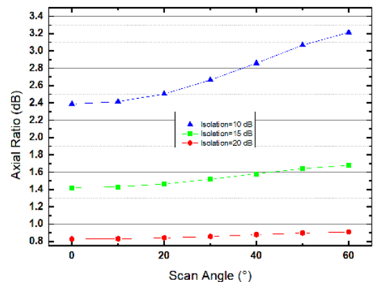
FIGURE 9. The variation in the axial ratio caused by beam steering.
