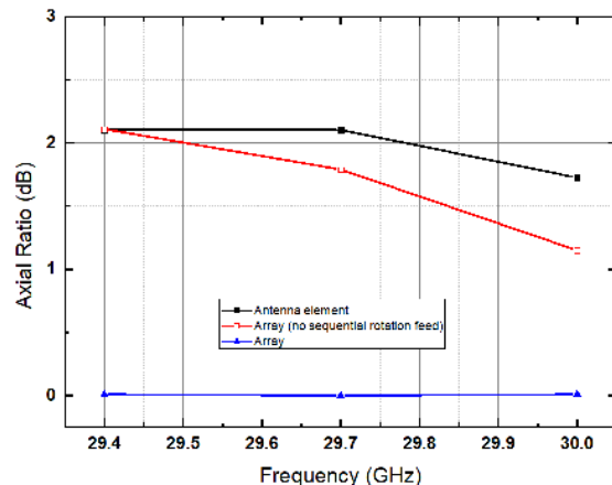
FIGURE 18. Simulated AR of the single element and 8 x 8 array.
