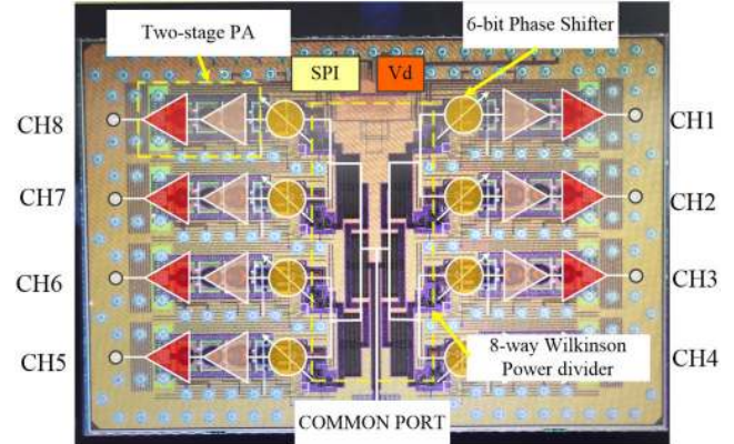
FIGURE 4. Architecture of the 8-channel transmit beamformer.
