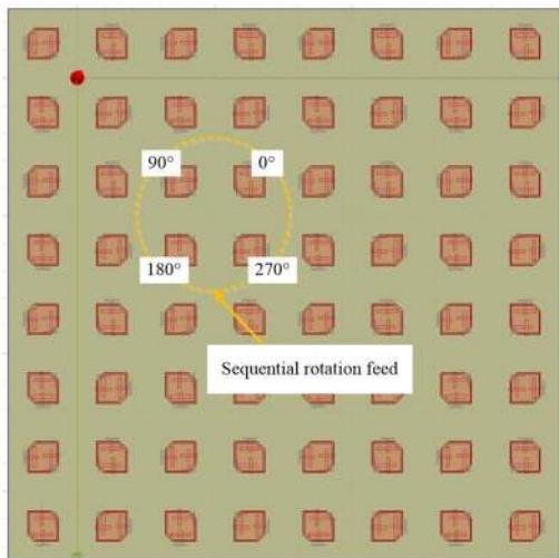
FIGURE 15. Simulation model of an 8 x 8-element array.
