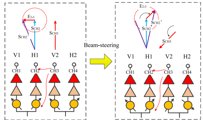
FIGURE 8. Coupling effect between adjacent channels.
