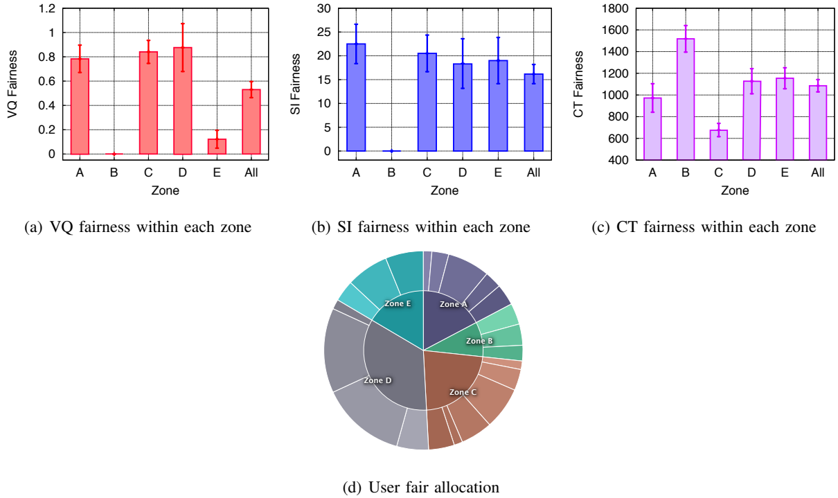
Fig. 10. Fairness measurements
