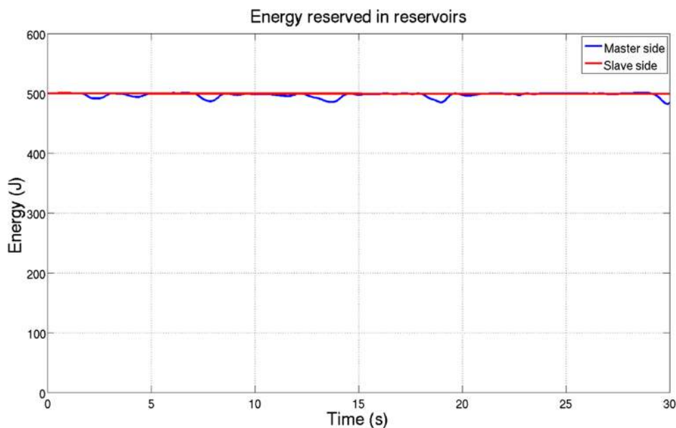
Fig. 33 Energy stored in the reservoirs of the WVC structure in free motion (energy reservoir 500J)
