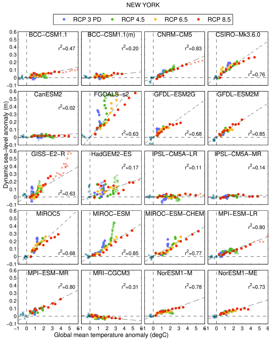
Fig. 2. Scatter plot of dynamic sea level change for New York City against the global mean surface air temperature anomaly (with respect to a 1980–1999 reference period; marker are 10-yr averages). The data represent the historical period (light blue crosses) and the four RCP scenarios (see legend). Stabilization periods (after 2100) are indicated with green crosses. During the stabilization period, the linear relationship between dynamic sea level change and global mean temperature is less robust, but this does not affect our projections towards the end of the 21st century. The dotted line is the linear regression over 2000–2100 based on all combined RCP scenarios, using yearly values. The r^2 score is also indicated on each panel, calculated from decadal averages between 2000 and 2100 (about 40 data points if all RCPs are available). The data are retrieved as the closest model grid cell from the geographical coordinates [40.5° N, 73.5° W].
