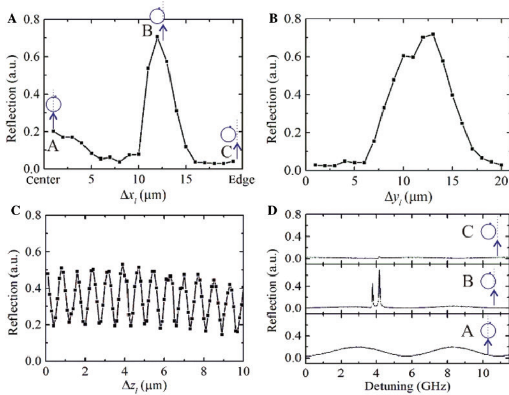
Figure 3: The amplitude of the reflection as a function of the spatial position of the GRIN lens (incident beam).
