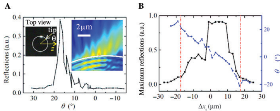
Figure 4: The amplitude of the reflection as a function of the spatial position of the microsphere and the nanotip.
