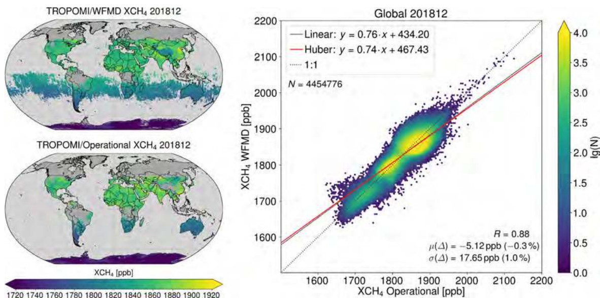
Figure 16. As Fig. 15 but for methane.
