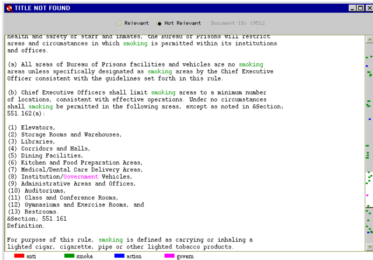
Figure 2. Scrollbar-based visualization
