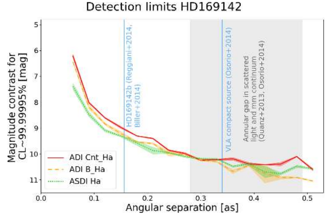
Fig. 9. Contrast curves for HD169142. The shaded region represents the annular gap observed in scattered light and in millimeter continuum (Osorio et al. 2014). The blue vertical lines represent the separation of the companion candidates (Reggiani et al. 2014; Biller et al. 2014; Osorio et al. 2014).
