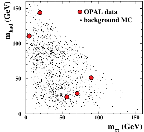
Fig. 6. The position in the (m_{\tau\tau}, m_{\text{had}}) plane of the h^0 A^0 \rightarrow \tau^+\tau^-q\bar{q} channel candidates, superimposed on that of the arbitrarily normalised expected Standard Model background, for \sqrt{s} = 161 and 170–172 GeV
