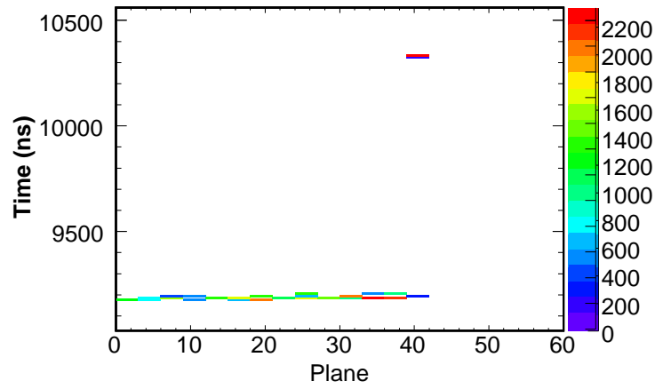
Figure A.12: The longitudinal position versus time of slices 8 and 9.
