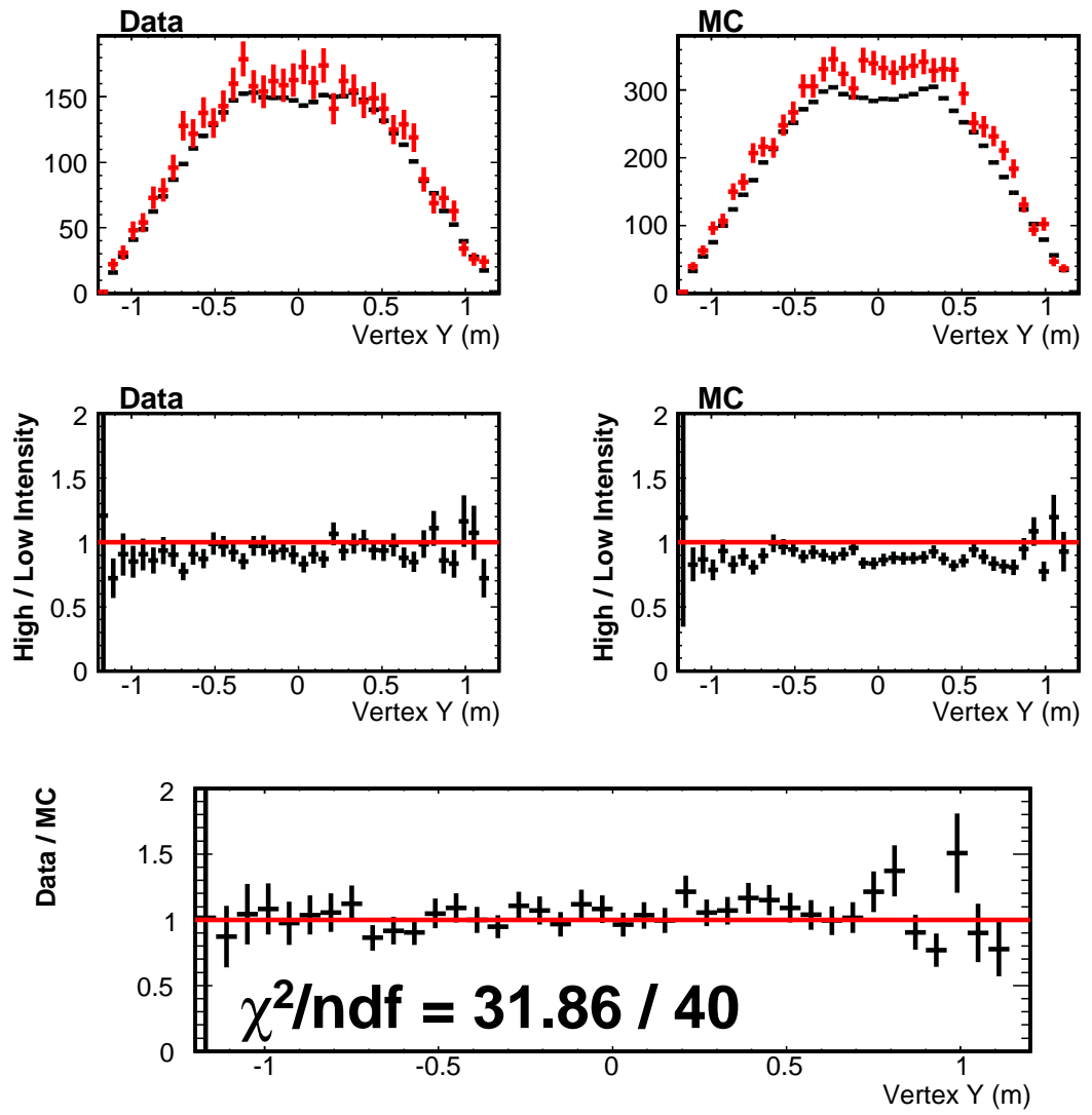
Figure 6.28: Reconstructed Y vertex for all events.
