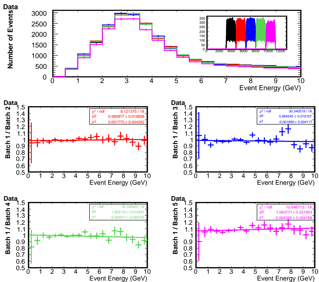
Figure 6.39: Charged current energy spectra from different NuMI batches. The top plot is the overlay of the different energy spectra for five different batches, given by the superimposed legend. The bottom four plots are the ratios of the spectra from the first batch to the others. Note the last batch has less protons on target than the other four so one does not necessarily expect a ratio of one.
