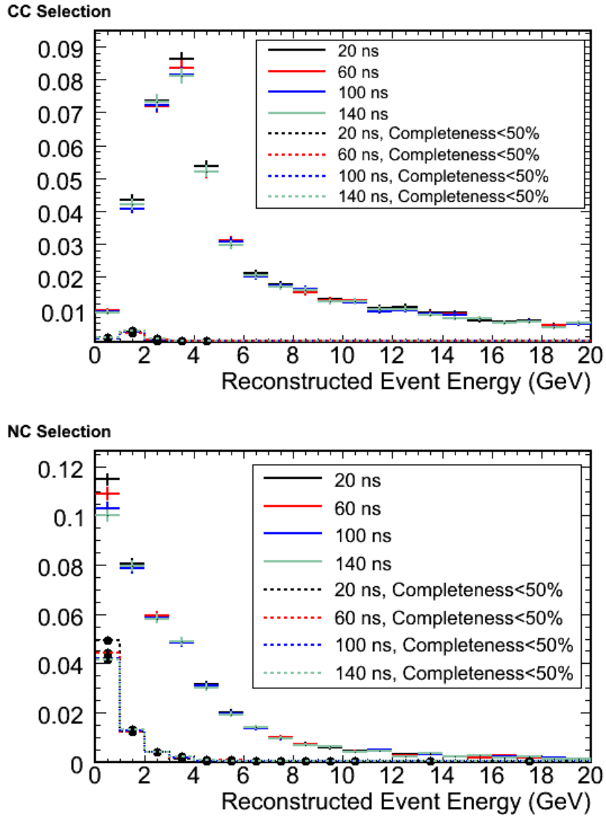
Figure 4.6: The charged current and neutral current energy spectra for different timing steps in the Slicing algorithm. The solid lines are the entire energy spectrum, while the dashed lines are the component of events that have a completeness less than 50%.
