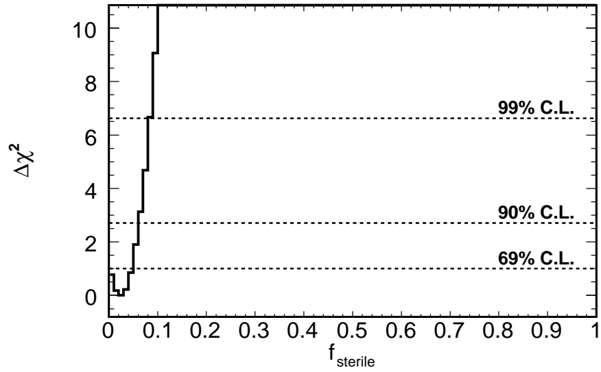
Figure 8.21: Oscillation results from the first MDC set. The top plot is the 2-D contour for f_{sterile} vs \Delta m^2 with 69%, 90%, and 99% confidence levels superimposed. The bottom plot is the 1-D contour for f_{sterile}
