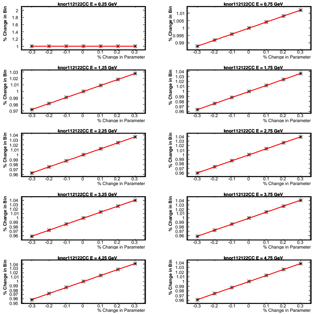
Figure 8.3: Fractional Change in the Neugen Parameter knor112122 versus Fractional Bin Content Change for CC-like events from 0-5 GeV Energy Bins
