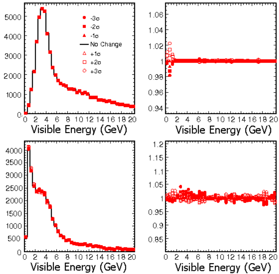
Figure B.5: The effect of changing kno_{r_{213223}} by \pm 1, 2, 3 \sigma .
