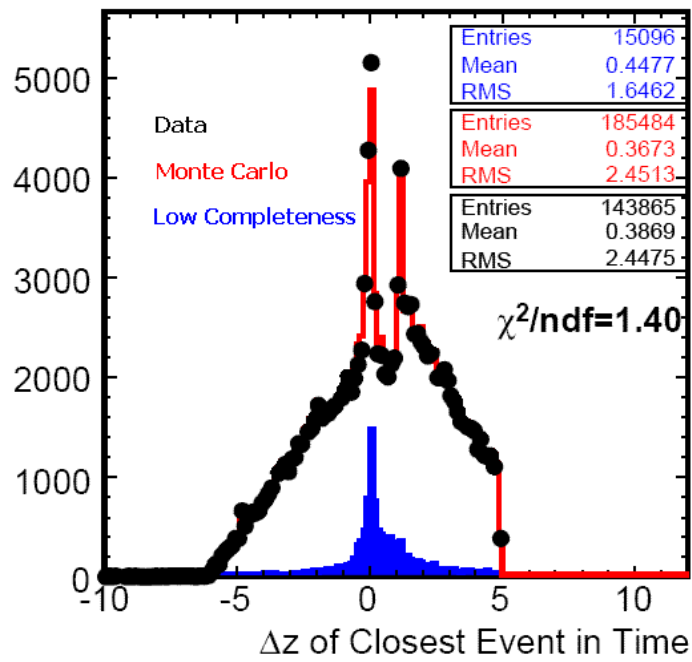
Figure 5.3: The top plot is a distribution of the minimum separation between two events in time. The bottom plot is a spatial distribution of the minimum distance in Z between two events. The black is data, the red is the Monte Carlo and the blue portion is the low completeness fraction of the Monte Carlo.
