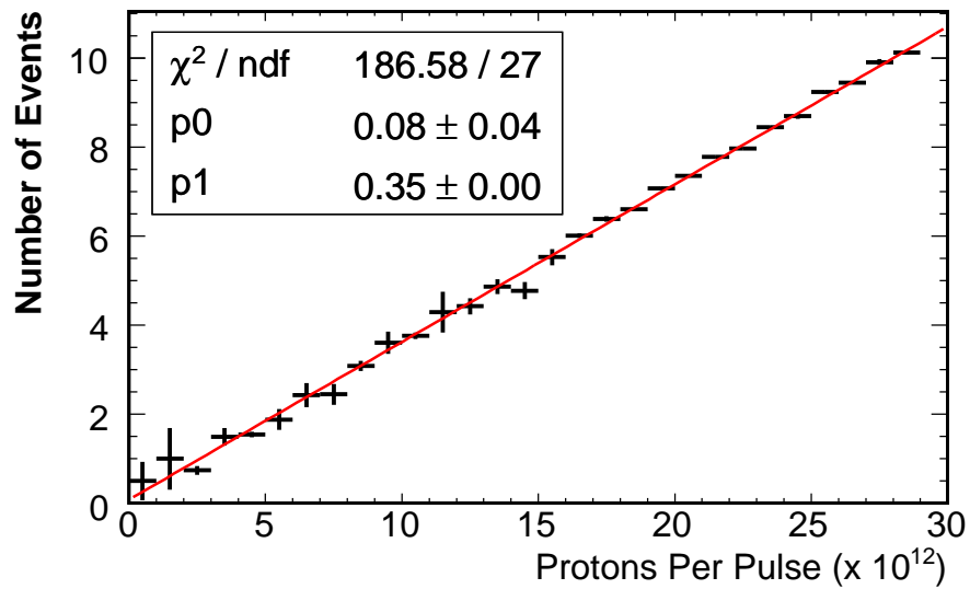
Figure 6.13: A plot of beam intensity ( \times 10^{12} protons per pulse) versus the average number of reconstructed slices in the top plot and the average number of reconstructed events in the bottom plot.)
