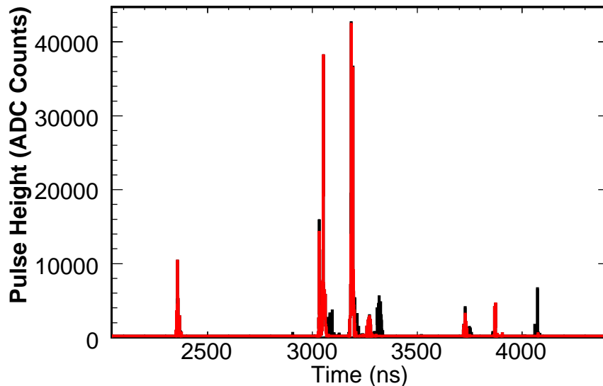
Figure 4.3: The timing distribution of a selection of hits in a 10\mu\text{s} neutrino spill. The black hits are all hits that occurred in the time interval, and the red is the same distribution with strips removed that had a pulse height less than 2 photoelectrons and in the spectrometer section.
