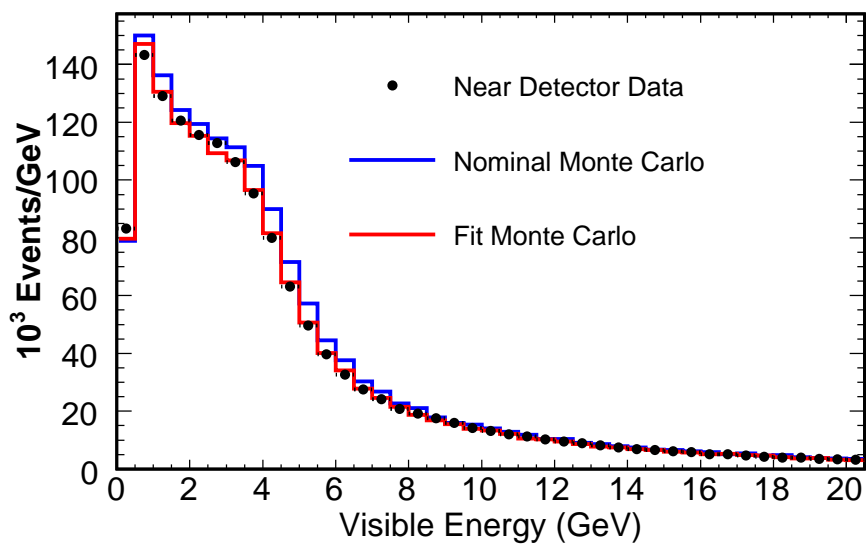
Figure 9.8: Results of fitting the Near detector charged current (top) and neutral current energy spectra (bottom). The black dots are the Near detector data, the blue spectra is the nominal Monte Carlo, and the red spectra is the best fit Monte Carlo to the data.
