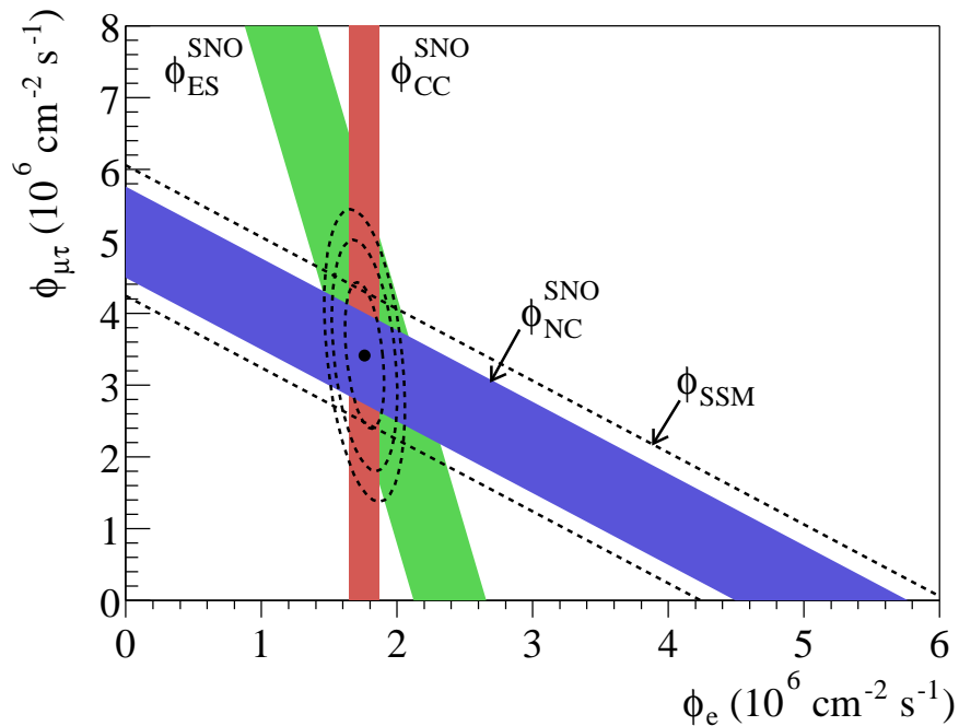
Figure 1.5: Flux {}^8\text{B} solar neutrinos which are \mu or \tau flavor vs flux of electron neutrinos deduced from the three neutrino reactions in SNO. the diagonal bands show the total {}^8\text{B} flux as predicted by the Standard Solar Model (dashed lines) and that measured with the NC reaction in SNO (solid band). The intercepts of these bands with the axes represent the \pm 1\sigma errors. The bands intersect at the fit values for the \phi_e and \phi_{\mu\tau} , indicating that the combined flux results are consistent with neutrino flavor transformation assuming no distortion in the {}^8\text{B} neutrino energy spectrum [22].
