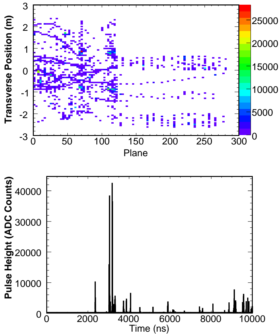
Figure 4.2: The top plot is a typical Near detector spill with an intensity of 2.42 \times 10^{13} protons per pulse. Each point is a individual strip in the detector and the color denotes pulse height in ADC counts. The z-axis is the plane number and the y-axis is the transverse position (m) in the detector. The bottom plot is the pulse height weighted timing distribution of all the strip hits in the detector. Each spike corresponds to some activity or interaction.
