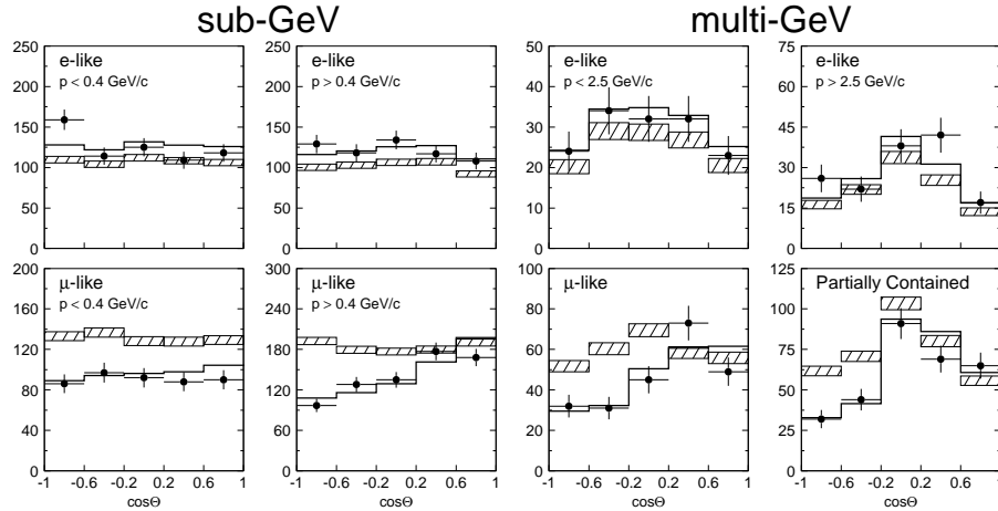
Figure 1.3: Zenith angle distributions of \mu -like and e -like events for sub-GeV and multi-GeV data sets. Upward-going particles have \cos\Theta < 0 and downward-going particles have \cos\Theta > 0 . Sub-GeV data are shown separately for p < 400 MeV/ c and p > 400 MeV/ c . Multi-GeV e -like distributions are shown for p < 2.5 GeV/ c and p > 2.5 GeV/ c and the multi-GeV \mu -like are shown separately for FC and PC events. The hatched region shows the Monte Carlo expectation for no oscillations normalized to the data live-time with statistical errors. The bold line is the best-fit expectation for \nu_\mu \leftrightarrow \nu_\tau oscillations with the overall flux normalization fitted as a free parameter [21].
