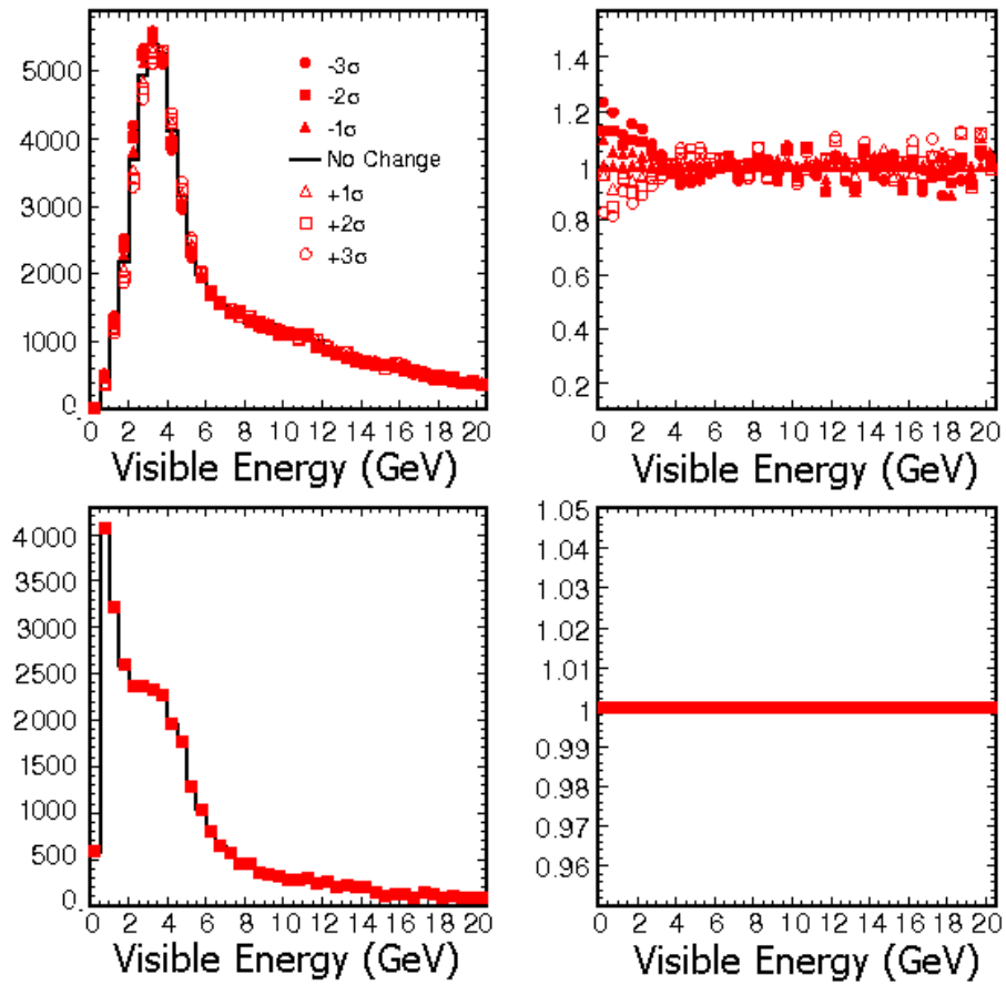
Figure B.10: The effect of changing the track energy by \pm 1, 2, 3 \sigma .
