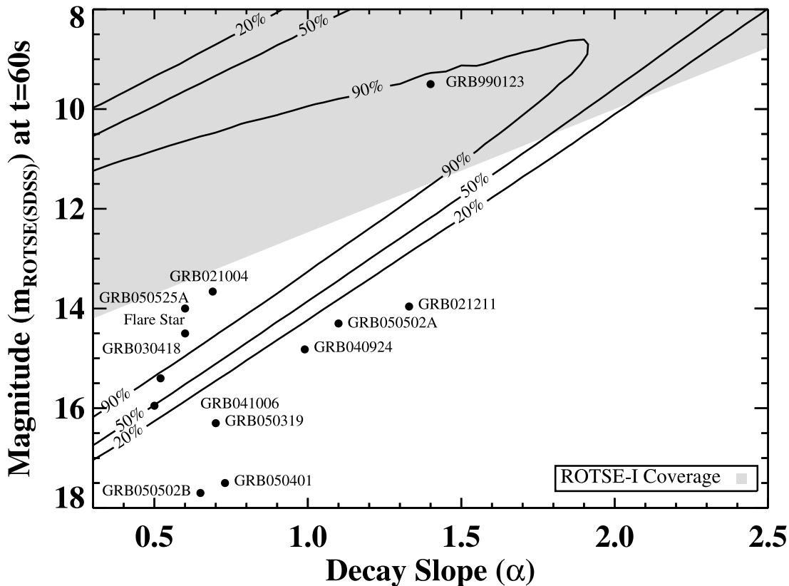
FIG. 5.—Detection efficiency for fading transients, parameterized by their peak magnitude at t = t_0 + 60 \text{ s} , m_{60} , and their decay constant \alpha . The efficiencies calculated assume 30 minutes of effective coverage for each set for an integrated coverage of 1.74 \text{ deg}^2 \text{ yr} . All sets with limiting magnitudes deeper than 17.5 were used for this plot. The contours describe our 20%, 50%, and 90% efficiency levels. The contours roll over at the bright end, where many transients would be saturated and rejected. The gray area describes the coverage in the ROTSE-I transient search. Overplotted are approximate peak magnitudes and decay constants (averaged over the first hour) for six GRB afterglows with early detections (Akerlof et al. 1999; Fox et al. 2003, 2004; Li et al. 2003; Rykoff et al. 2004b, 2005a, 2005b, 2005c; Yost et al. 2005; Falcone et al. 2005).
