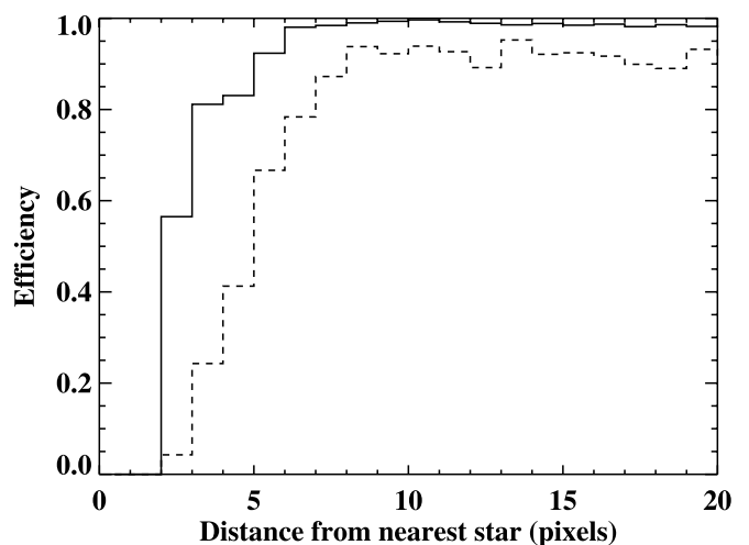
FIG. 2.—Detection efficiency in a pair of images vs. distance from nearest template star. The solid line describes simulated objects more than 0.5 mag brighter than the limiting magnitude; the dashed line describes simulated objects within 0.5 mag of the limiting magnitude, where our detection efficiency is reduced.
