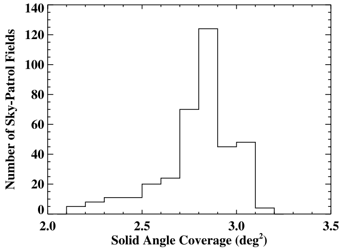
FIG. 3.—Histogram of solid angle coverage for our sky patrol fields. The maximum available solid angle in our field is 3.42 \text{ deg}^2 , and the efficiency in most of the fields is >80\% .
