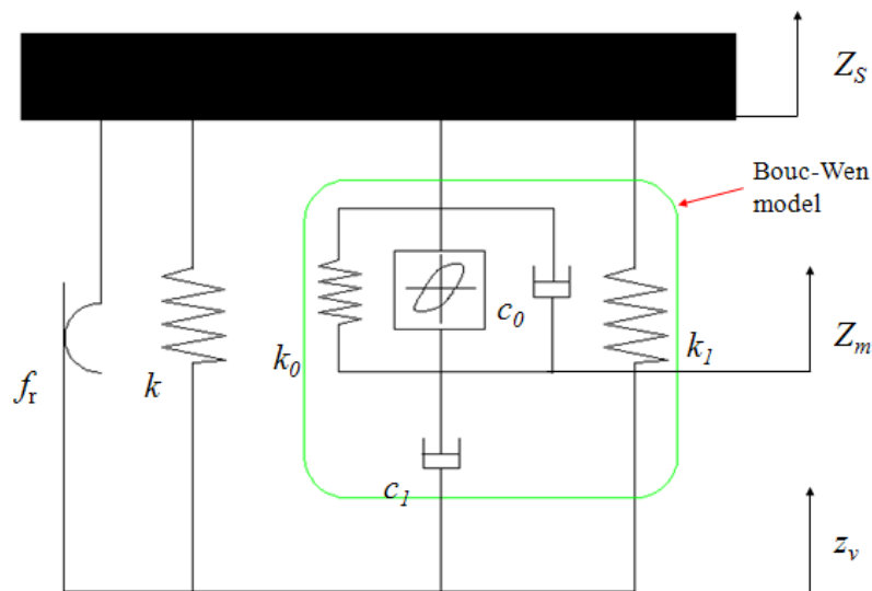
Fig.6. The mathematic model of seat suspension
