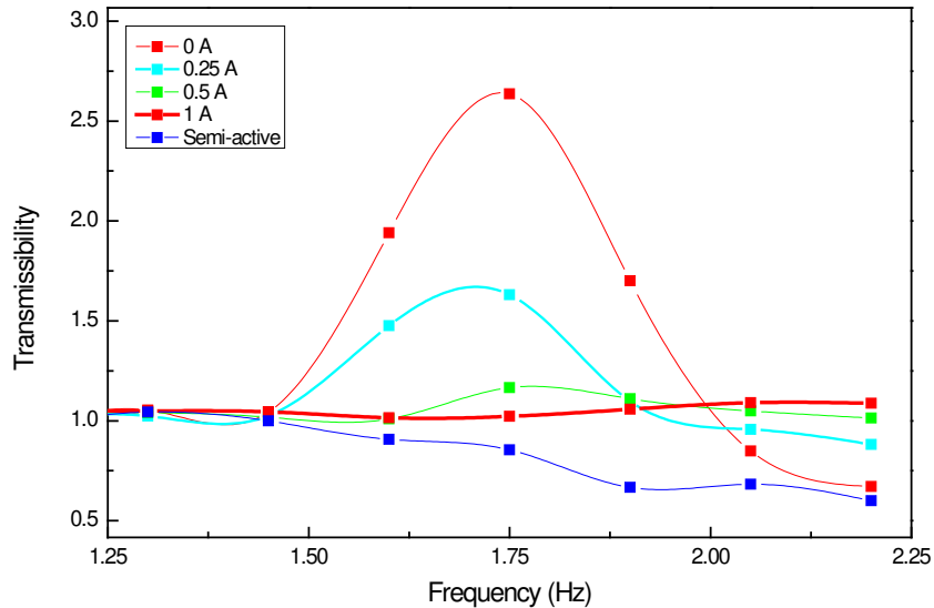
Fig.12 The transmissibility of the MR seat suspension under different frequencies
