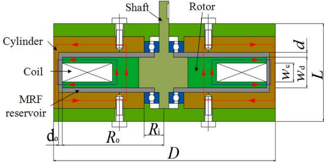
Fig. 2 The structure of the rotary MR damper
