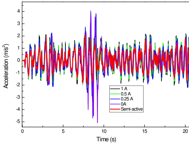
Fig.13 The performance of MR seat suspension under random excitation
