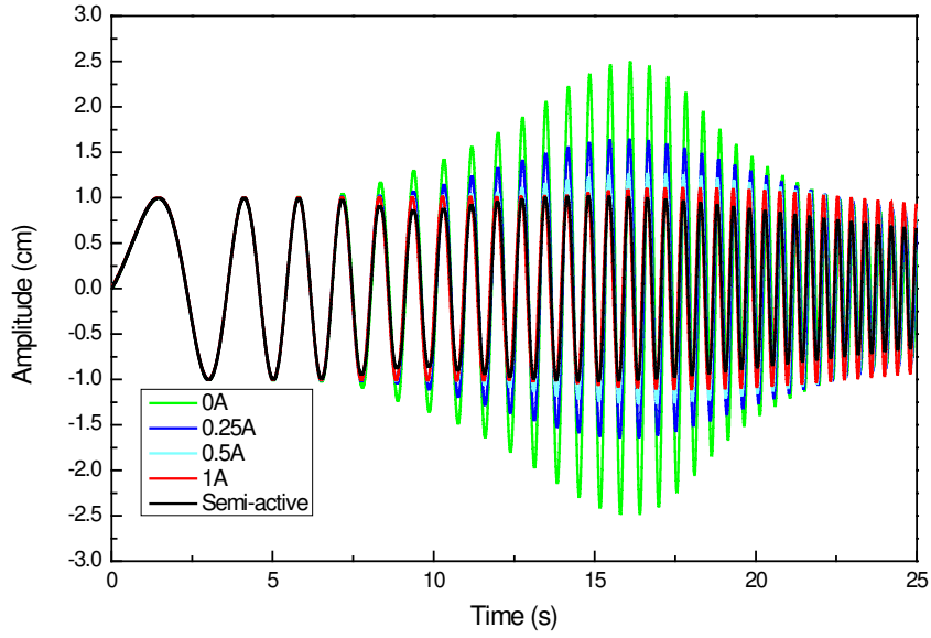
Fig.8 The simulation response of seat under harmonic excitation
