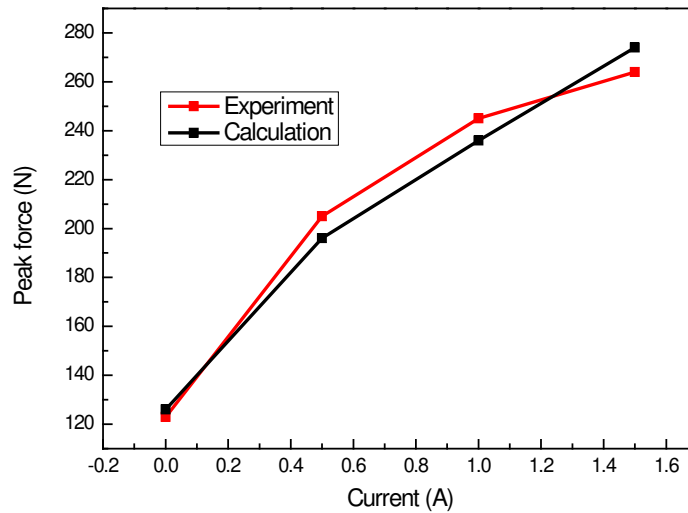
Fig. 5 The comparison between the experimental peak force and calculated peak force
