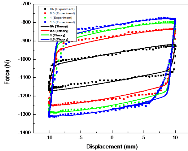
Fig. 7 The fitting result of the mathematic model
