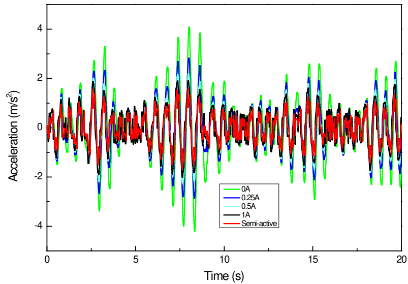
Fig.9 The simulation response of seat under random excitation
