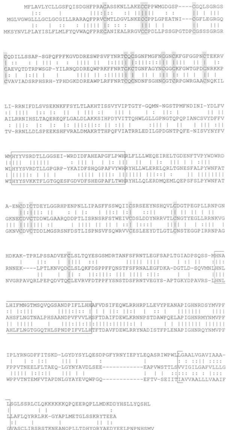
Fig. 5. Sequence comparison of tyrosinase-related protein family. The sequences of mouse tyrosinase (top row), TRP-2/DT (middle) and TRP-1 (lower) aligned to maximize amino acid similarity. Identical amino acids are indicated by | and amino acids with chemically similar properties by . The 15 conserved cysteine residues are shaded, the two copper binding sites are boxed and the hydrophobic transmembrane domain is enclosed by brackets.
