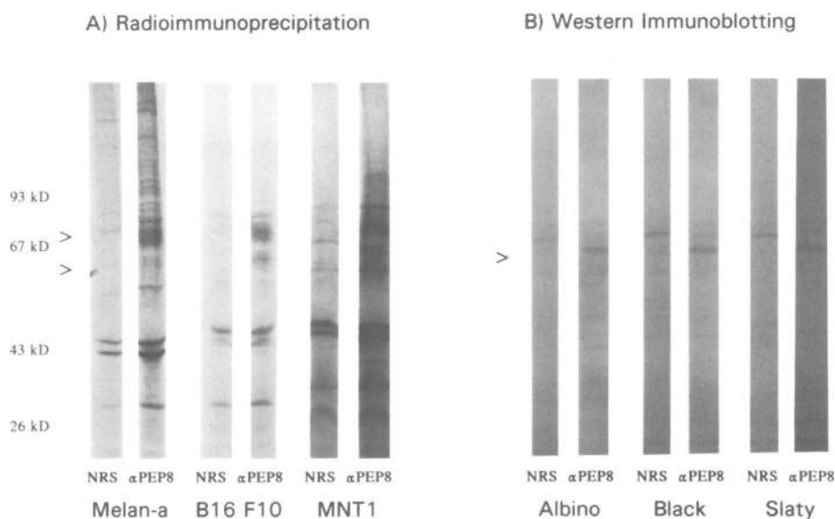
Fig. 4. Expression of TRP-2/DT protein. (A) Immunoprecipitation of labelled peptides from wild-type mouse melanocytes (melan-a), wild-type mouse melanoma (B16 F10) and human melanoma (MNT 1) cells. Precipitations were carried out using normal rabbit serum (NRS) or antibodies specifically directed against the C-terminus of TRP-2 ( \alpha PEP8). The arrows indicate the unglycosylated precursor peptide of 55 kDa and the mature, glycosylated form of 75 kDa both seen in the \alpha PEP8 lanes, but not the NRS. (B) Western blot detection of TRP-2/DT in eye extracts of albino , black (wild-type, C57BL/6J) and slaty (congenic with C57BL/6J) mice, reacted with normal rabbit serum (NRS) and with antibodies against the C-terminal peptide of TRP-2 ( \alpha PEP8).
