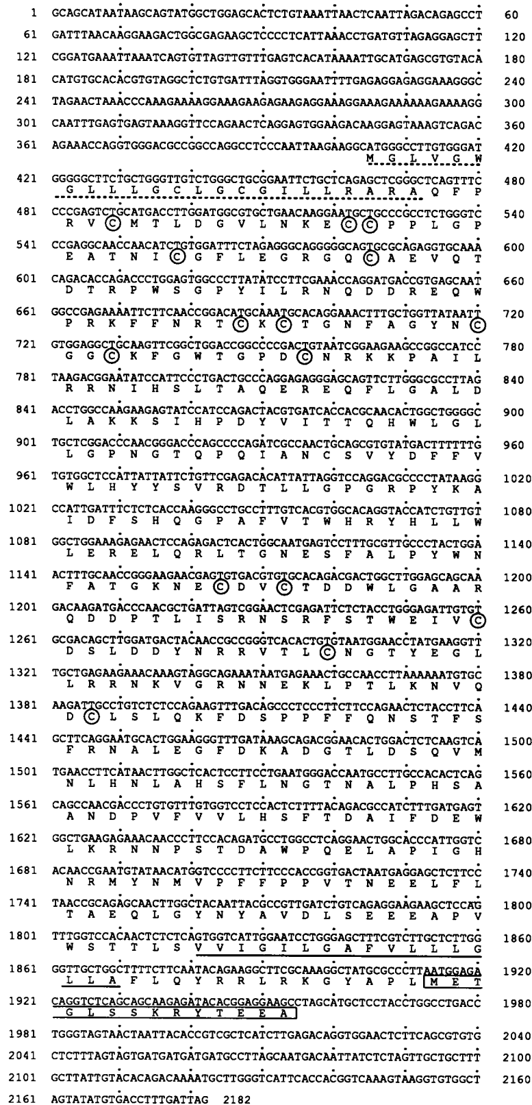
Fig. 1. Sequence of TRP-2 cDNA. The presumed full-length open reading frame is shown below the DNA sequence. All 15 cysteine residues (enclosed by circles) are conserved across the whole tyrosinase-related family. The N-terminal signal sequence is underlined with a dotted line, and the hydrophobic transmembrane domain has a solid underline. The boxed C-terminal 14 residue peptide (PEP8) was used to raise anti-TRP-2 antiserum. These sequence data are available from EMBL/GenBank/DBJ under accession number X63349.
