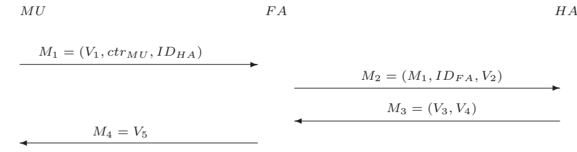
Fig. 1 Message Flows in login and Authentication Phase.
