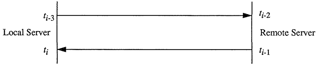
Figure 2. Computation of clock offset and roundtrip delay.
