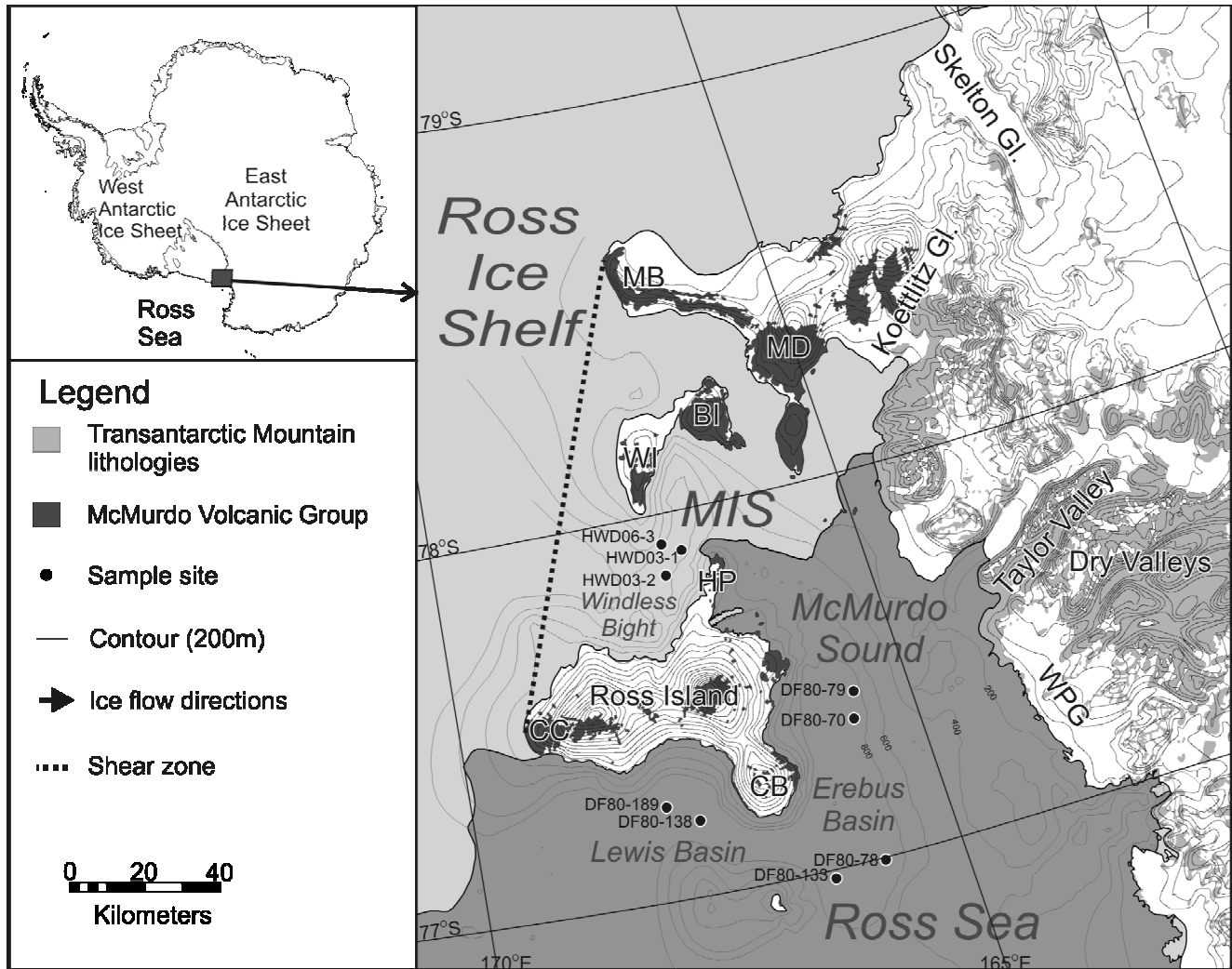
Figure 1 Map of Ross Island region showing the core sites and localities mentioned in text. The two main provenance areas and raised beaches locations (Dochat et al., 2000; Hall and Denton, 1999) discussed in text are also shown. BI = Black Island, CB = Cape Bird, CC = Cape Crozier, HP = Hut Point Peninsular, MB = Minna Bluff, MD = Mount Discovery, WI = White Island, WPG = Wilson Piedmont Glacier.
