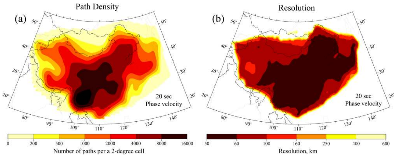
Figure 7. Examples of path density and resolution maps. (a) Path density estimated for the 20 s Rayleigh wave phase speed map in units of the number of paths contained in each 2° square cell ( \sim 50\,000\text{ km}^2 ). (b) Estimated resolution for the 20 s Rayleigh wave phase speed map, where resolution is defined as twice the standard deviation of the 2-D Gaussian fit to the resolution surface at each grid node.
