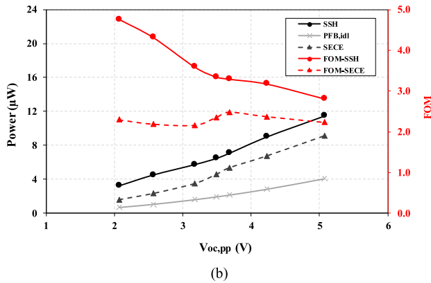
Fig. 17. Measured harvested power from custom-made MEMS PEH by the proposed IC compared to SECE IC and ideal full-bridge rectifier at different excitation levels ( C_P = 2 nF, C_{stor} = 1 μF).
