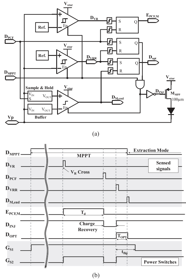
Fig. 11. (a) MPPT circuit and (b) corresponding signal waveforms.
