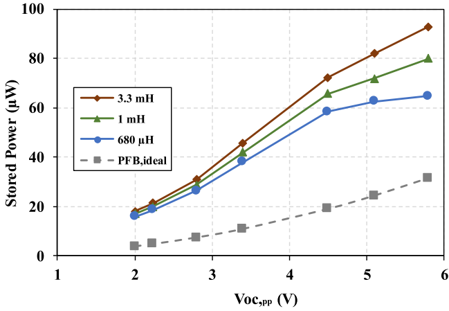
Fig. 16. Measured extracted power versus excitation OC piezoelectric voltage for three different external inductors (103YB PEH, C_P = 15 nF, L = 3.3 mH, C_{stor} = 1 μF).
