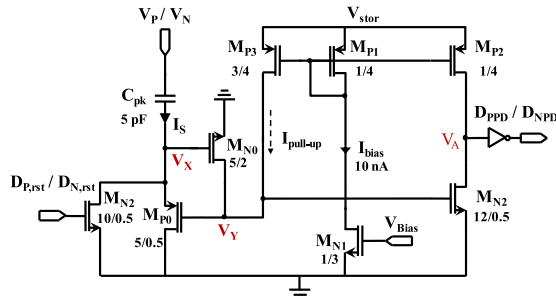
Fig. 8. Schematic of the implemented peak detector.
