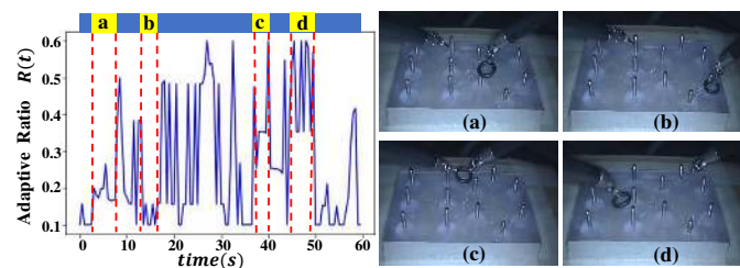
Fig. 5. An example of the evolution of the adaptive scaling motion ratio with typical surges during a trial. (a) S3: Move to Next Target with Right Hand (approach critical areas); (b) S2: Grasp Object with Right Hand (tool-tissue interaction); (c) S1: Transfer Object Operation (bimanual operation); (d) S6: Move to Next Target with Left Hand (far from critical areas).
