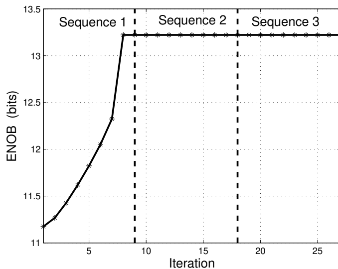
Fig. 8 Evolution of the Effective Number Of Bits (ENOB) during iterations -off line
