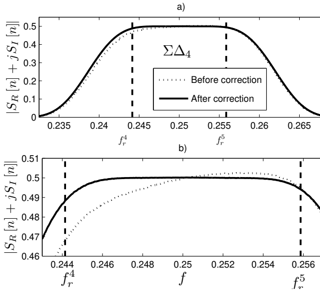
Fig. 15 First phase STF calibration
