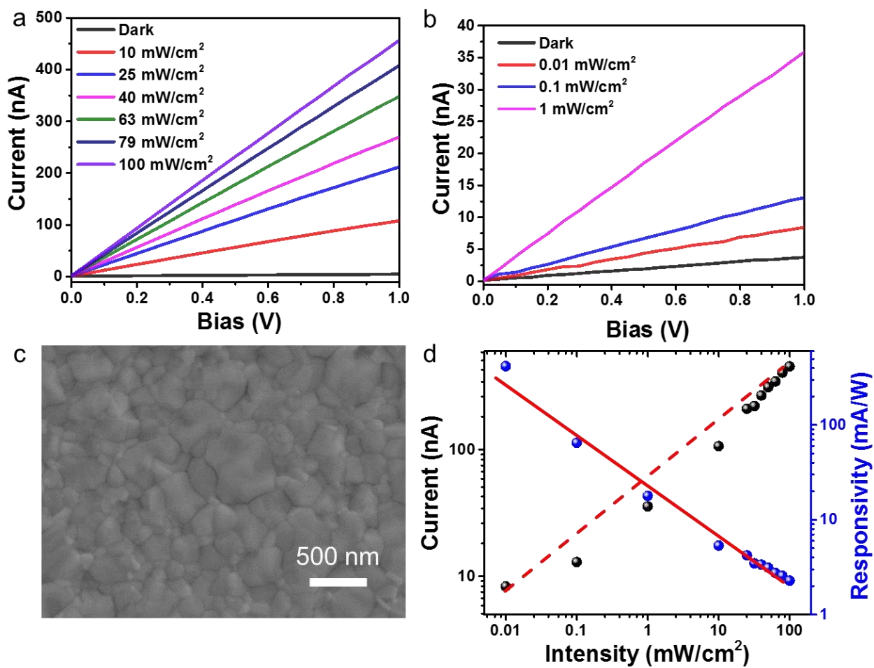
Figure 2. (a) I - V curves of the perovskite PD measured under various intensities of light, including (b) weak light conditions in conventional current detection mode. (c) Top-view SEM image of the high quality \text{CH}_3\text{NH}_3\text{PbI}_3 thin film processed with solvent-engineering. (d) Photocurrent and responsivity of the perovskite PD under various intensities of light.
