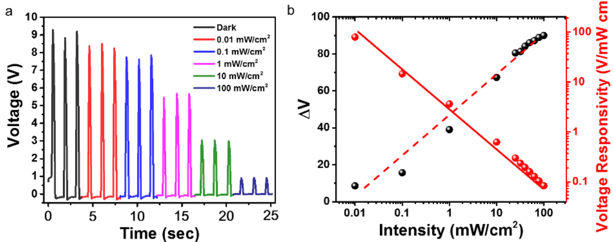
Figure 3. (a) The PD device voltage measured across the perovskite under various intensities of light in voltage detection mode. (b) The change in the measured voltage ( \Delta V ) and voltage responsivity of the device at different light intensities.
