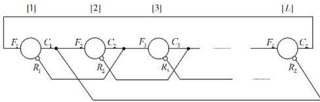
Fig. 5. Architecture of a self-timed ring
