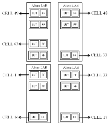
Fig. 9. Example of a self-timed ring (STR) topology for a 63-stage STR in Altera Cyclone III device (each Altera Logic Array Block -LAB- contains 16 logic cells consisting of a LUT and a flip-flop)
