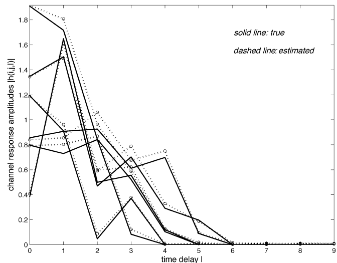
Fig. 4. Channel response amplitudes ( \text{SNR} = 21.4 dB).
