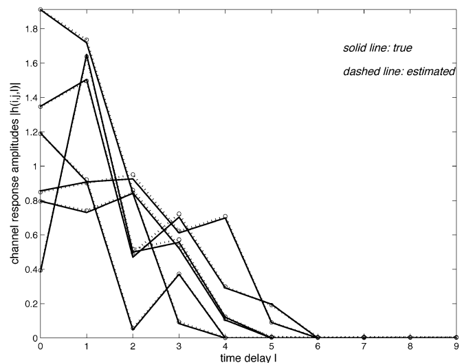
Fig. 5. Channel response amplitudes ( \text{SNR} = 28.5 dB).
