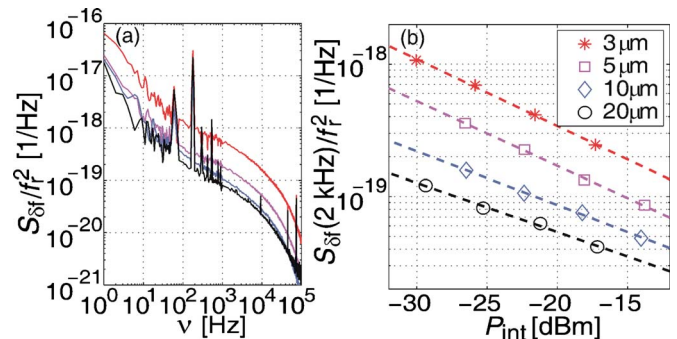
FIG. 1. (Color online) Fractional frequency noise spectra of the four CPW resonators measured at T=55 mK. (a) Noise spectra at P_{\mu w} = -65 dBm. From top to bottom, the four curves correspond to CPW center strip widths of s_r = 3, 5, 10 , and 20 \mu\text{m} . The various spikes seen in the spectra are due to pickup of stray signals by the electronics and cabling. (b) Fractional frequency noise at \nu=2 kHz as a function of P_{\text{int}} . The markers represent different resonator geometries, as indicated by the values of s_r in the legend. The dashed lines indicate power law fits to the data of each geometry.
